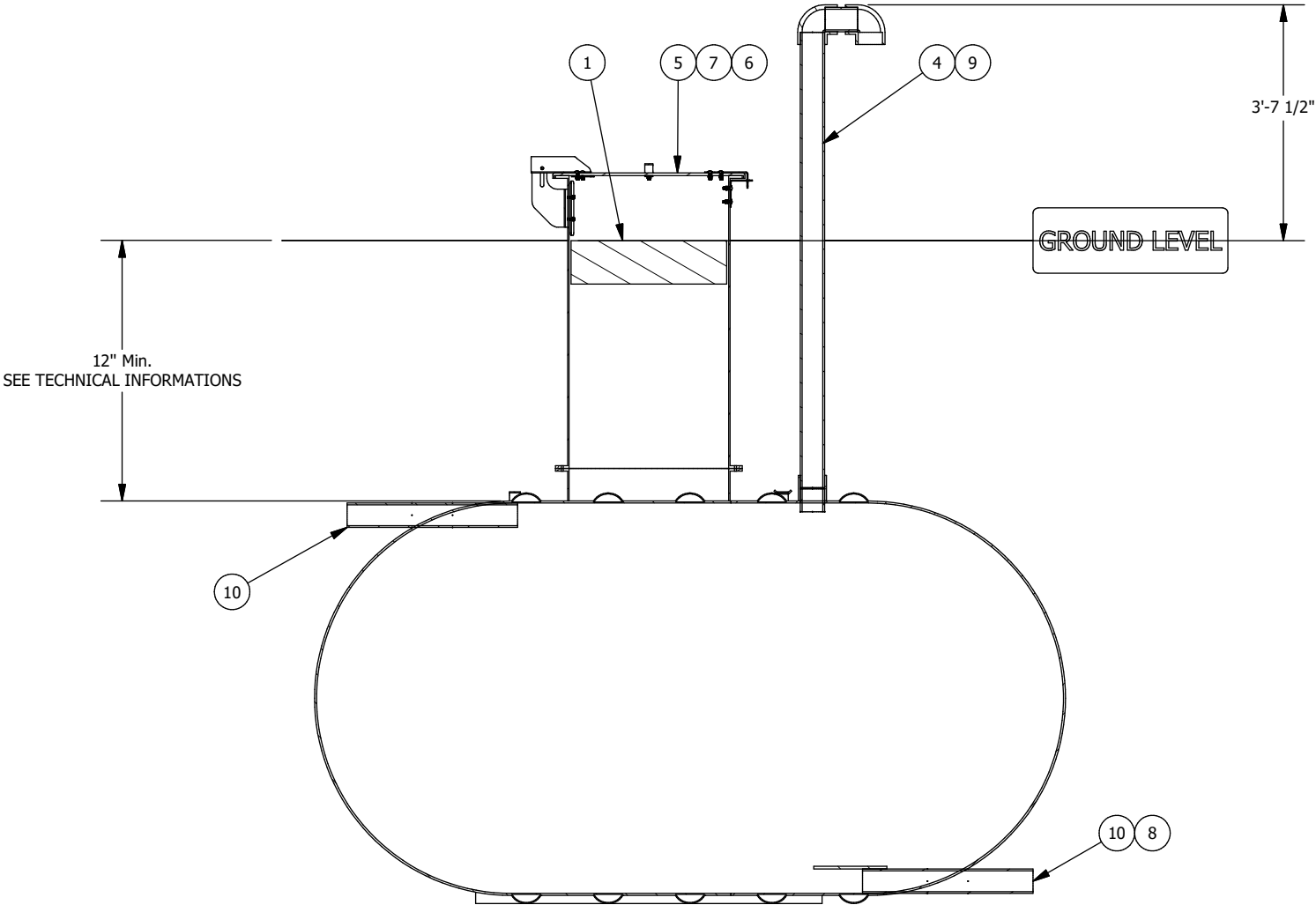
SECTION ELEVATION VIEW
