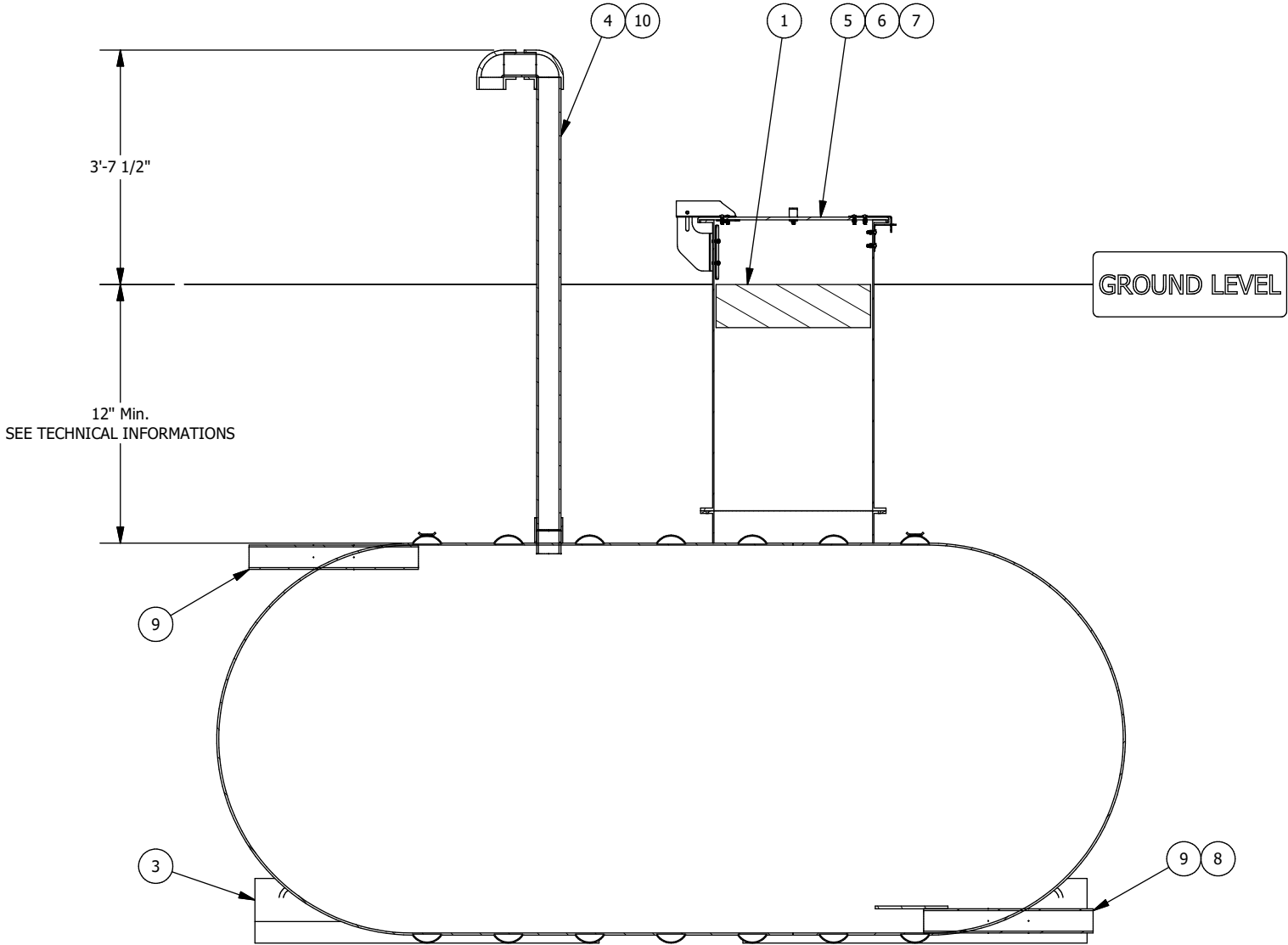
SECTION ELEVATION VIEW
