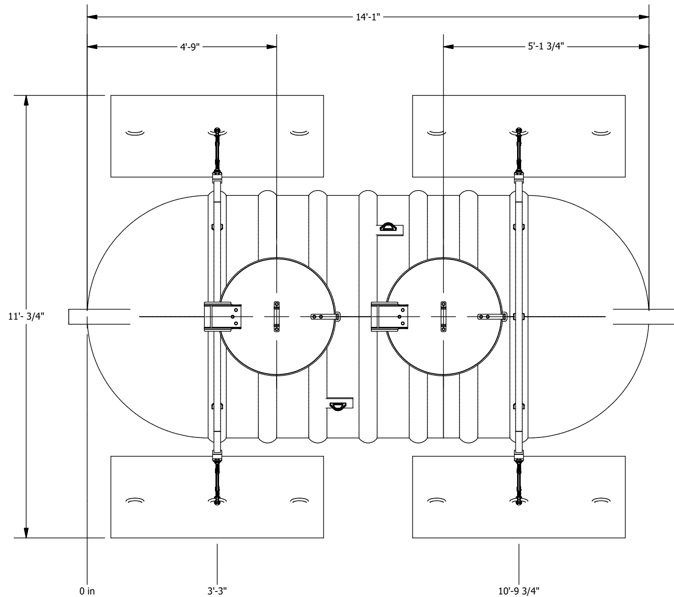
PLAN VIEW
