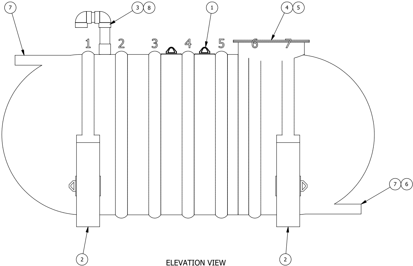
ELEVATION VIEW
