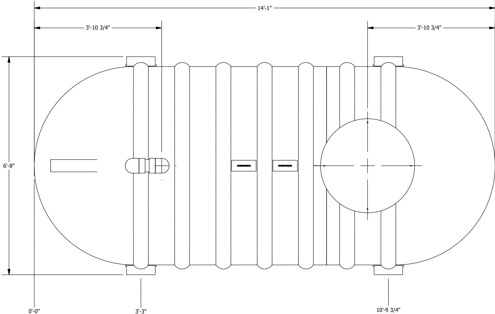
PLAN VIEW
