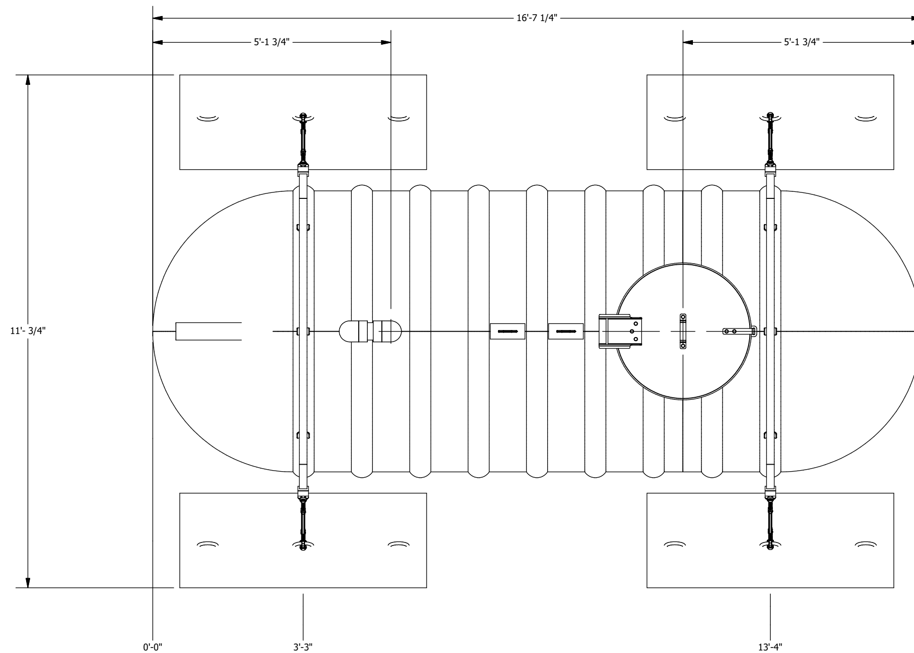
PLAN VIEW
