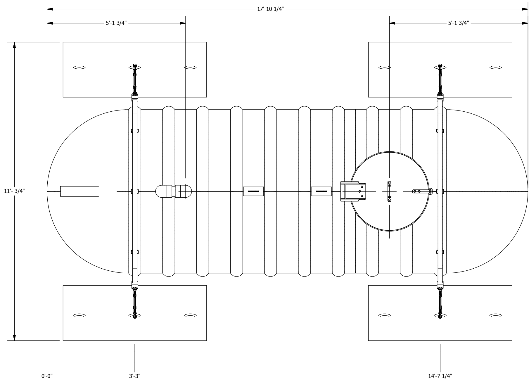
PLAN VIEW
