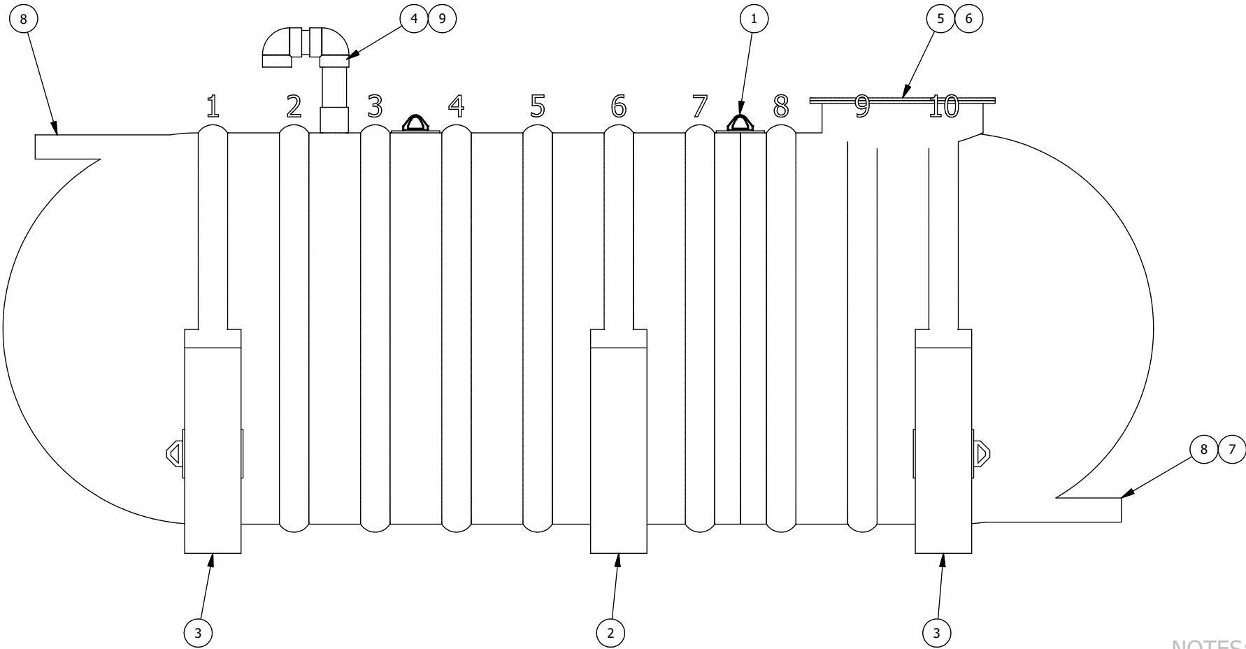
ELEVATION VIEW
