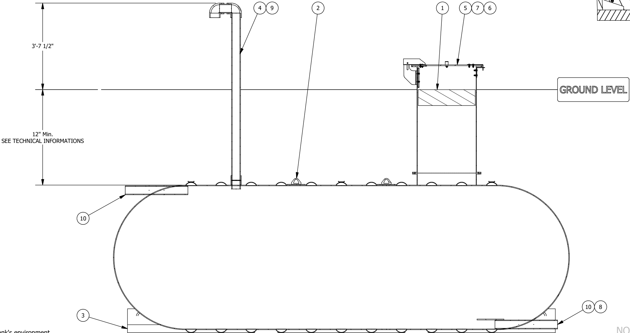
SECTION ELEVATION VIEW
