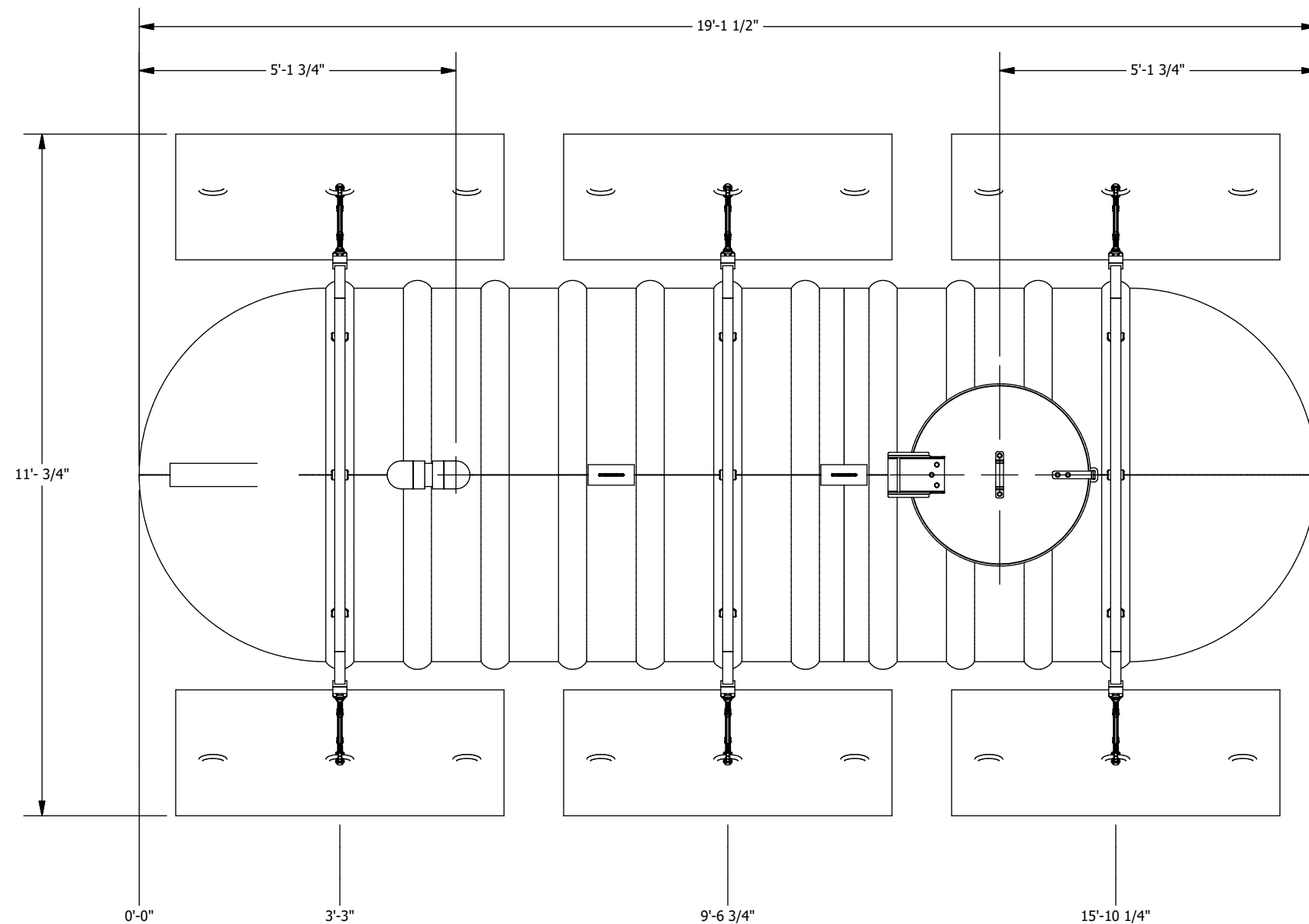
PLAN VIEW
