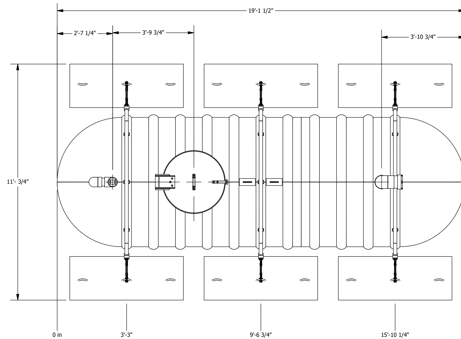
PLAN VIEW
