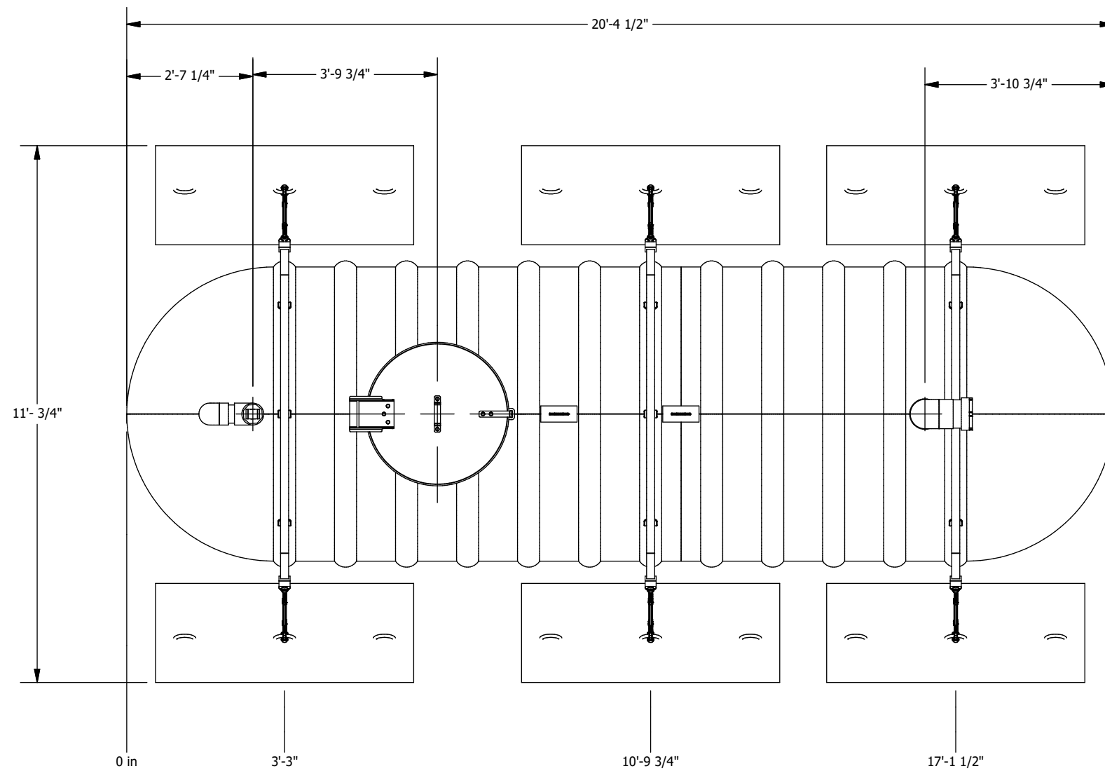
PLAN VIEW
