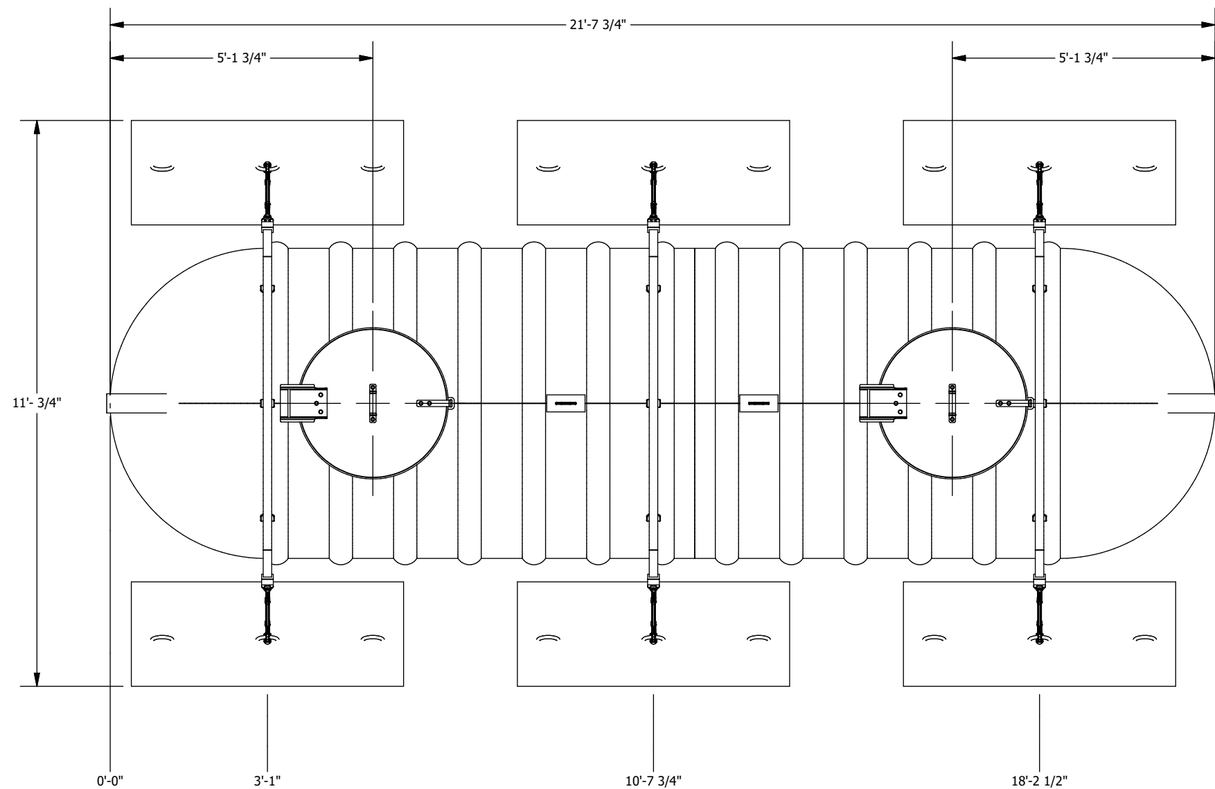
PLAN VIEW
