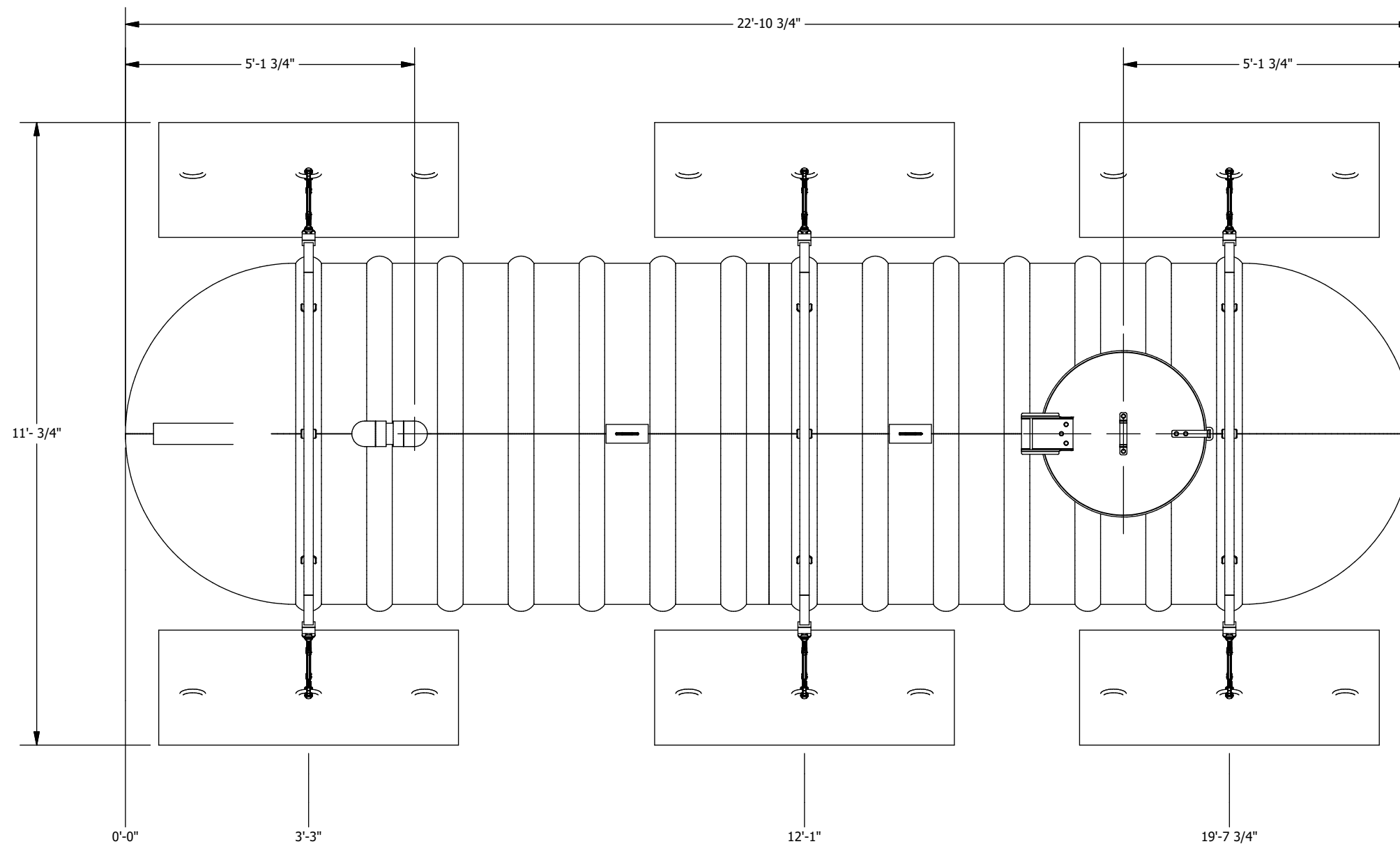
PLAN VIEW
