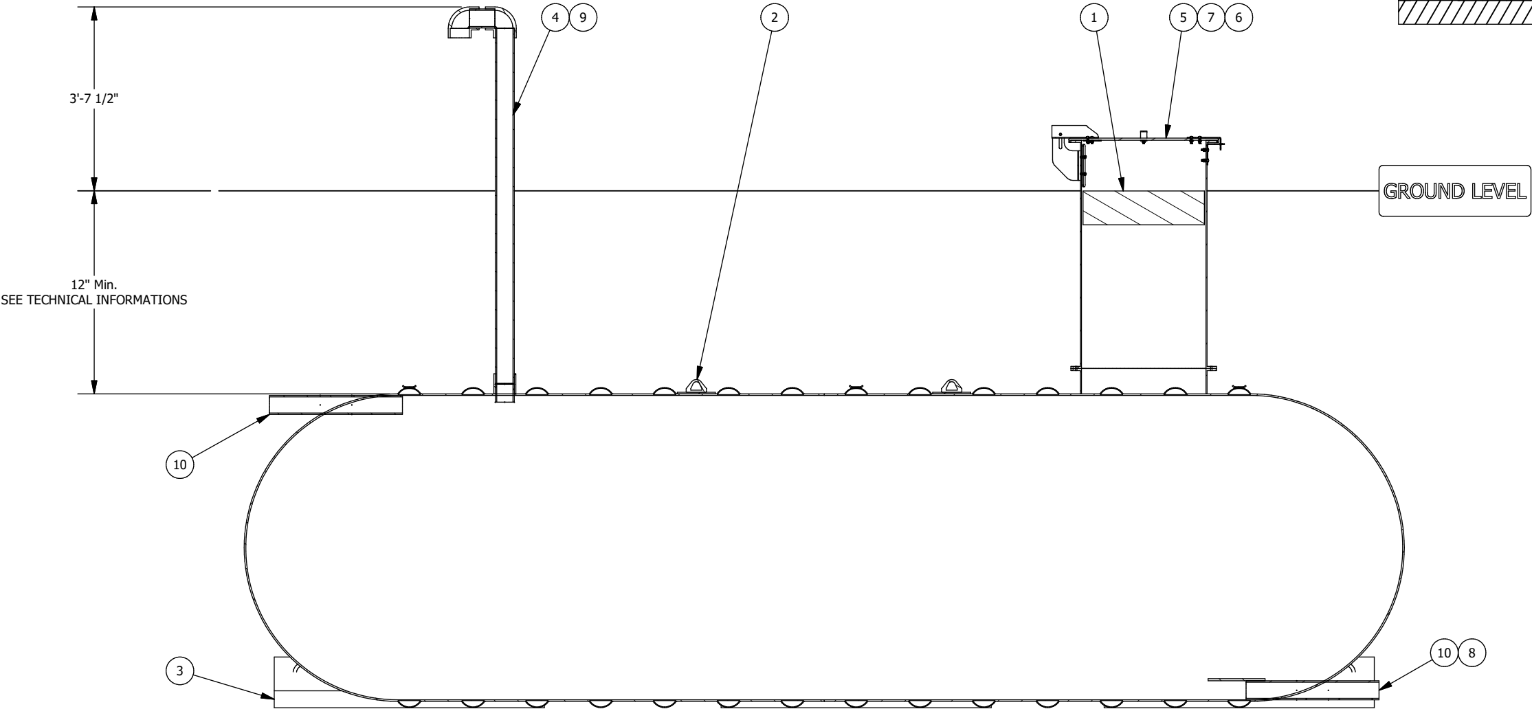
SECTION ELEVATION VIEW
