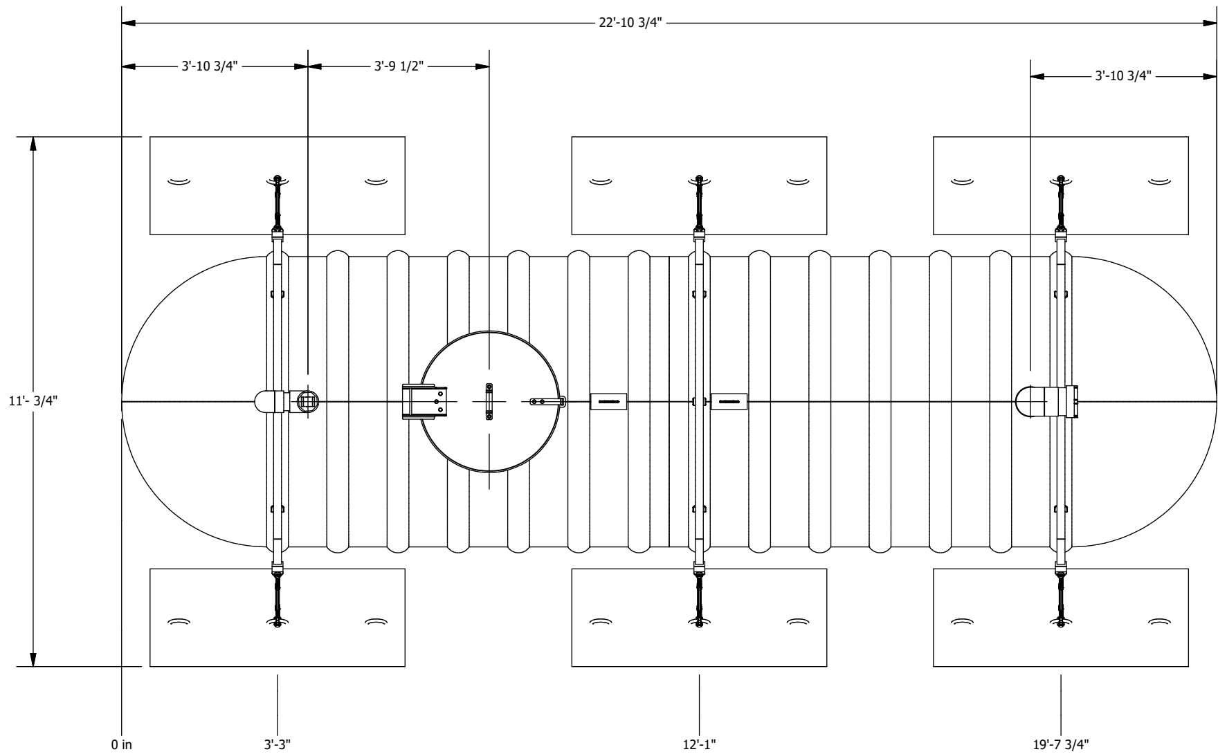
PLAN VIEW
