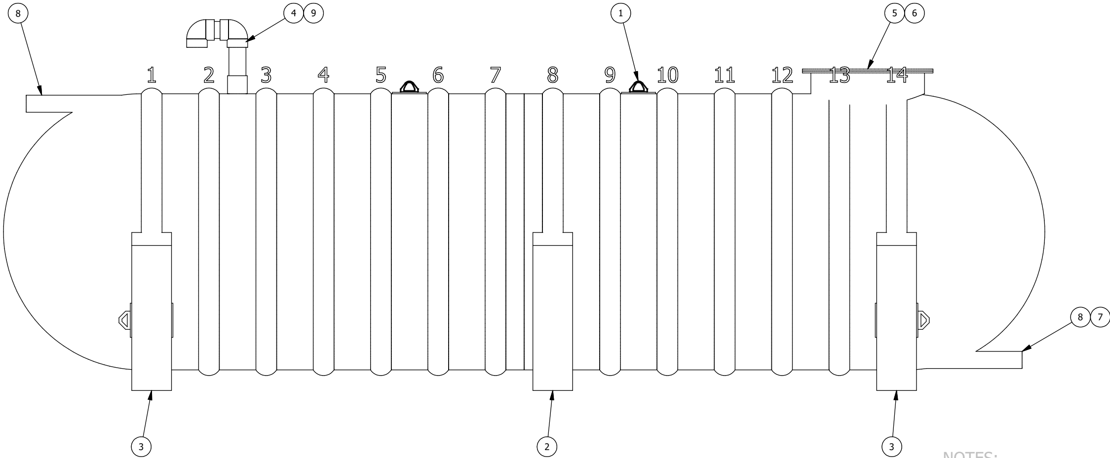
ELEVATION VIEW
