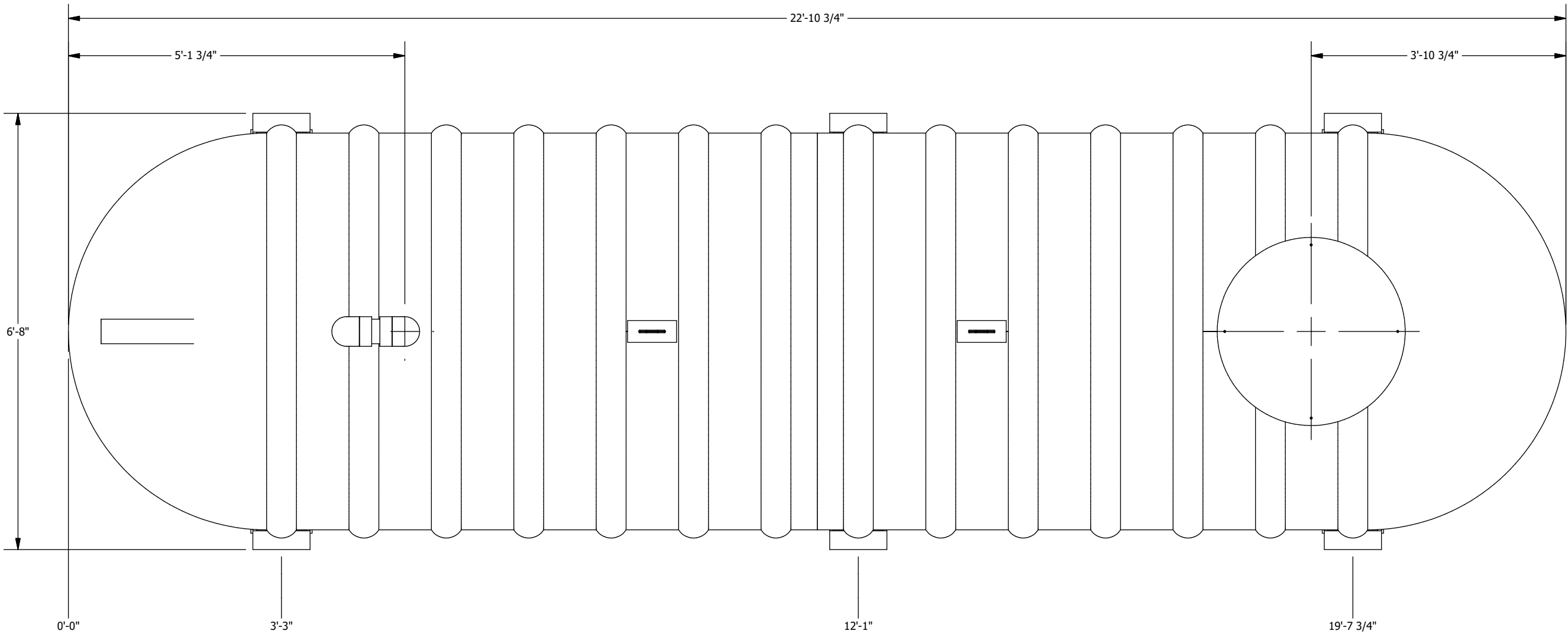
PLAN VIEW
