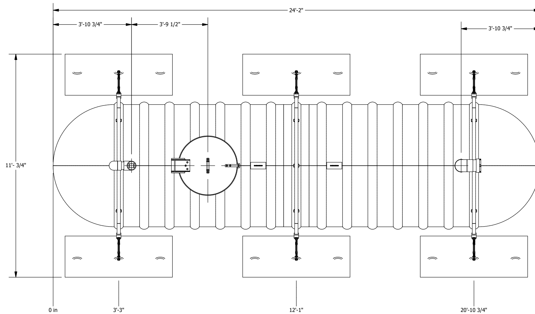
PLAN VIEW
