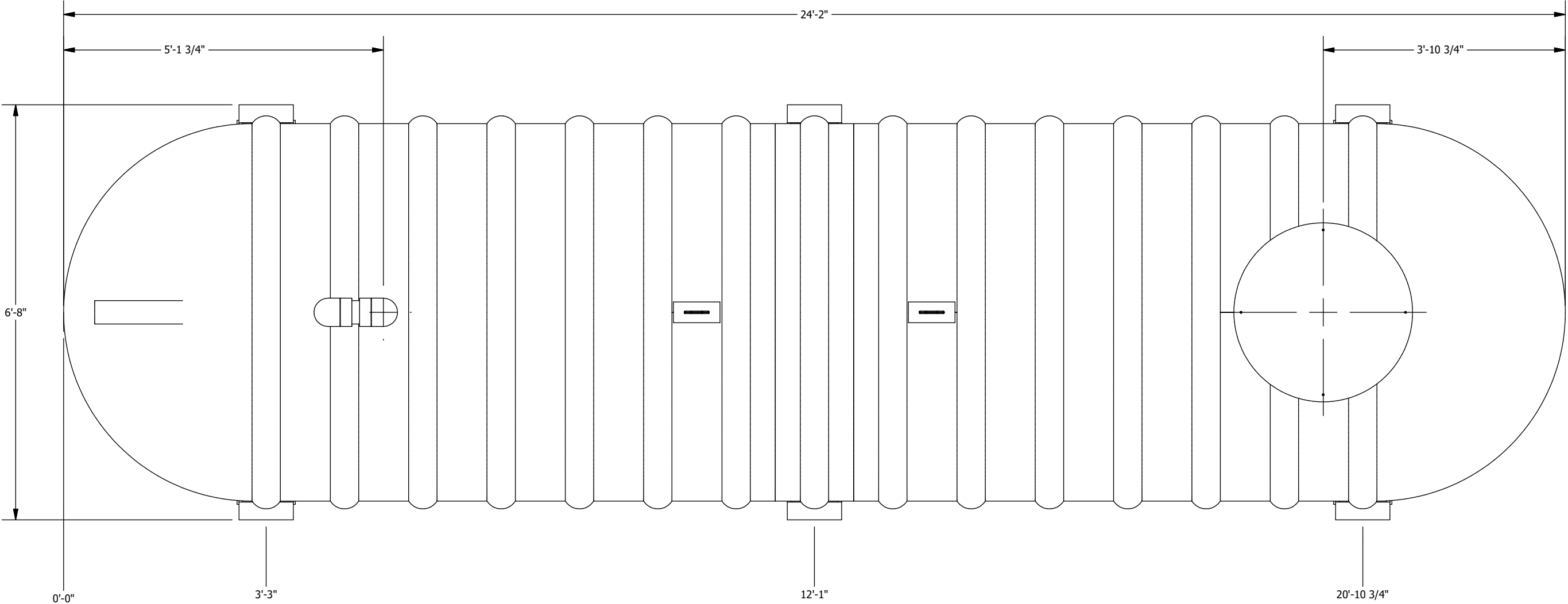
PLAN VIEW
