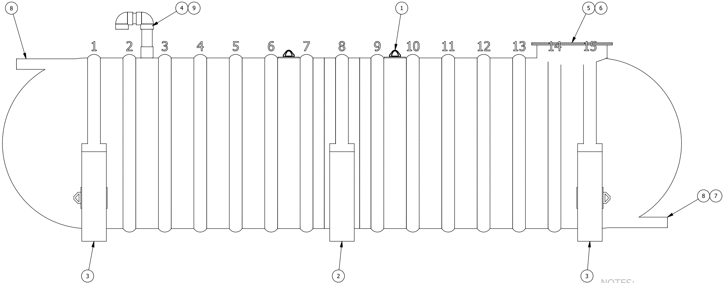
ELEVATION VIEW
