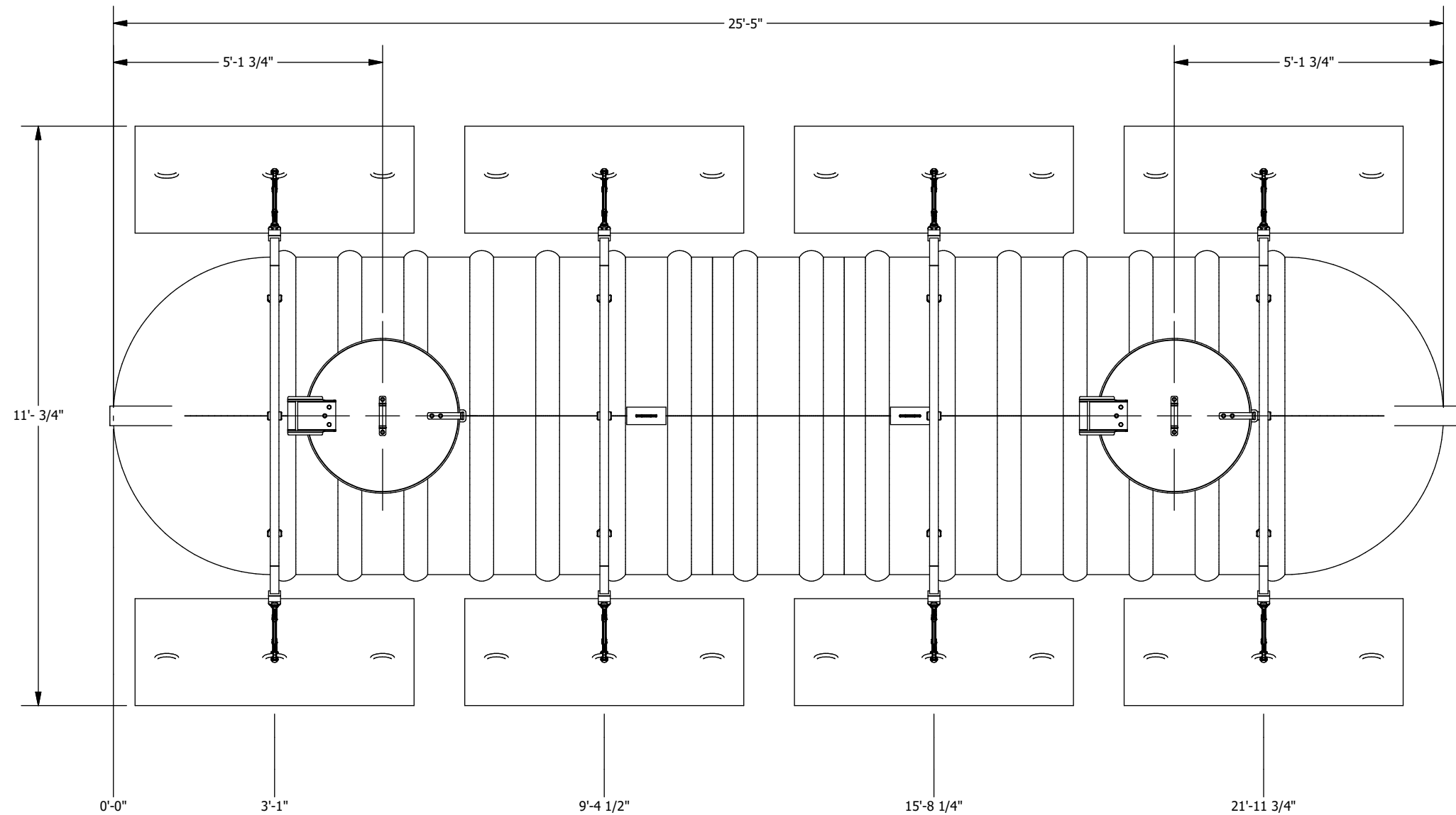
PLAN VIEW
