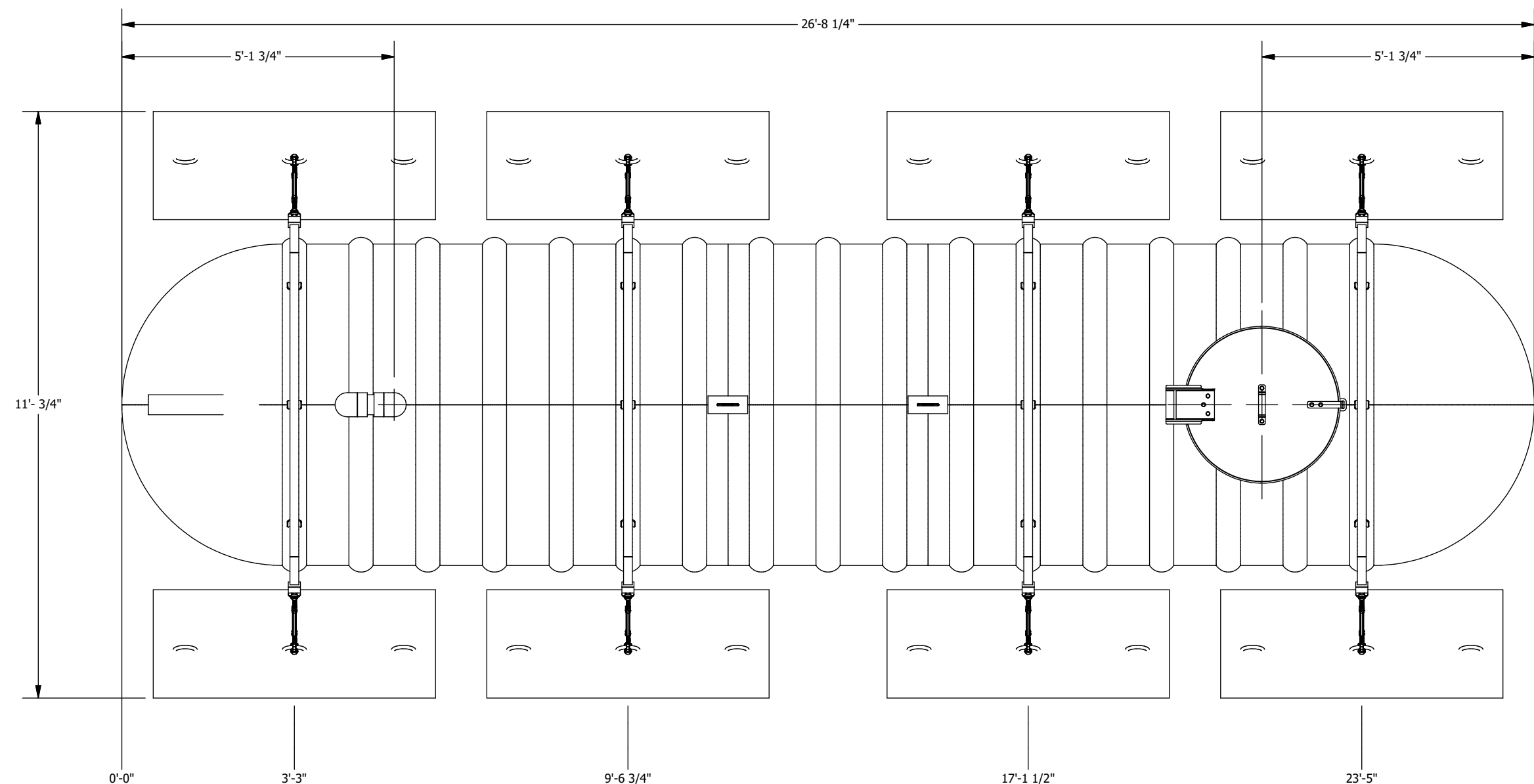
PLAN VIEW
