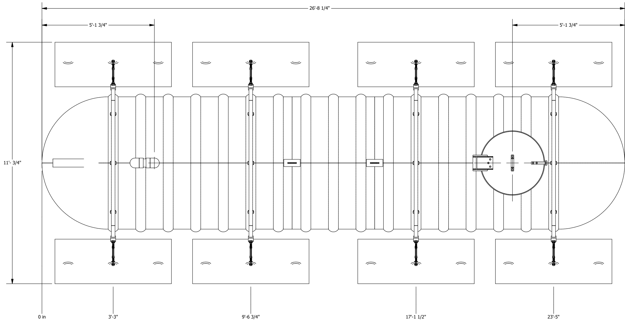
PLAN VIEW
