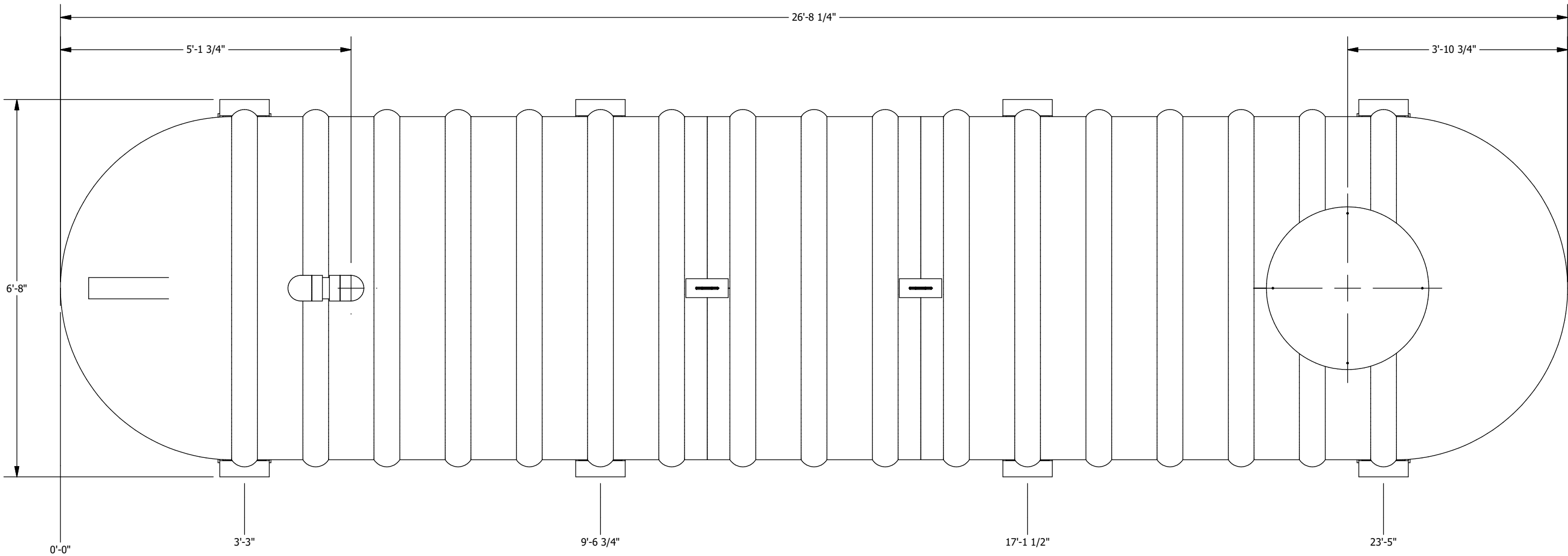
PLAN VIEW
