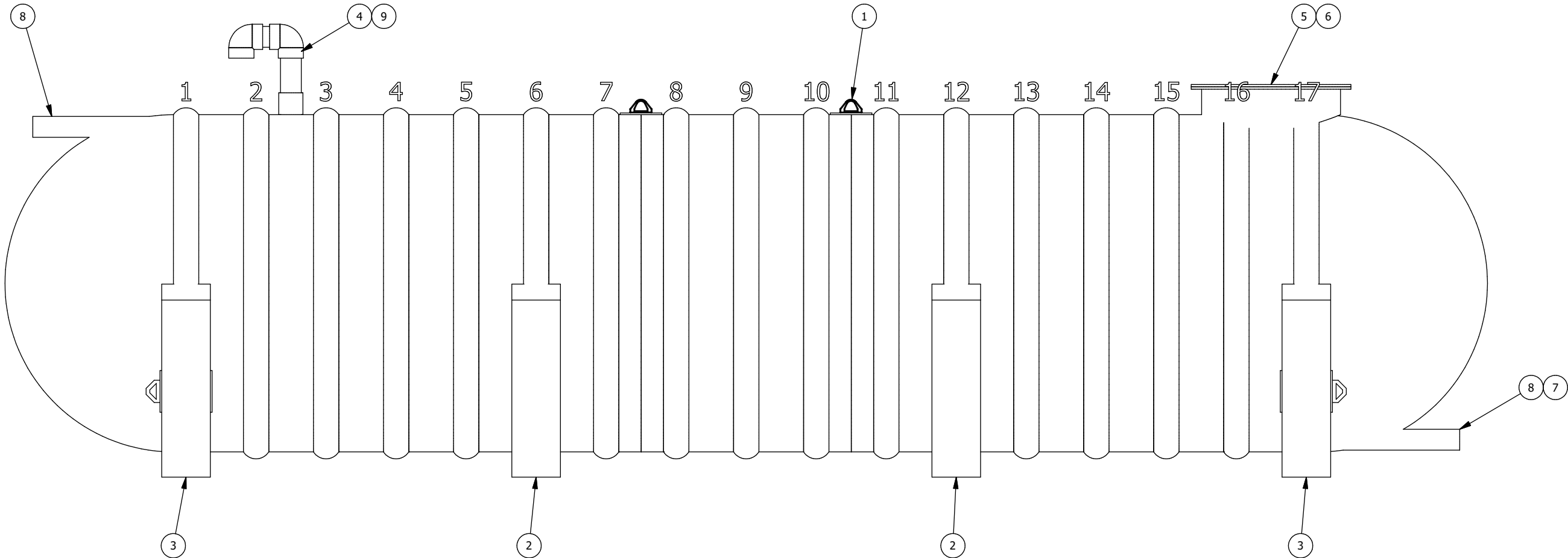
ELEVATION VIEW
