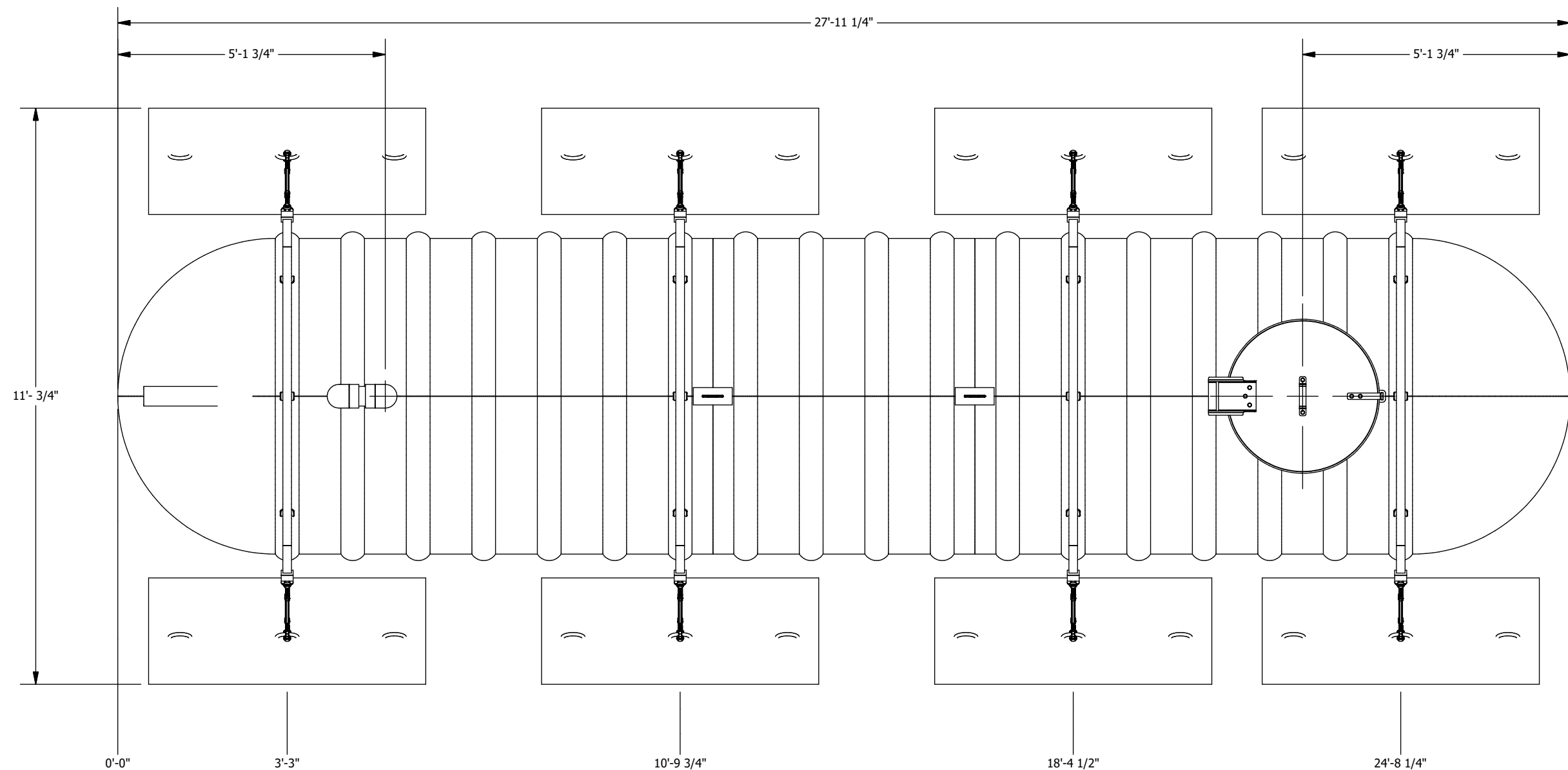
PLAN VIEW
