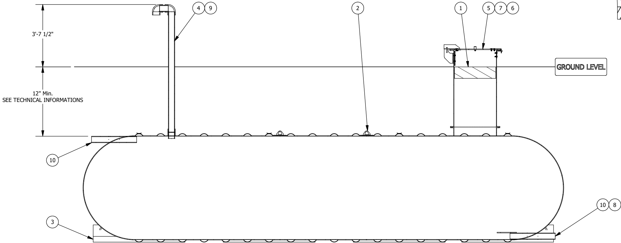
SECTION ELEVATION VIEW
