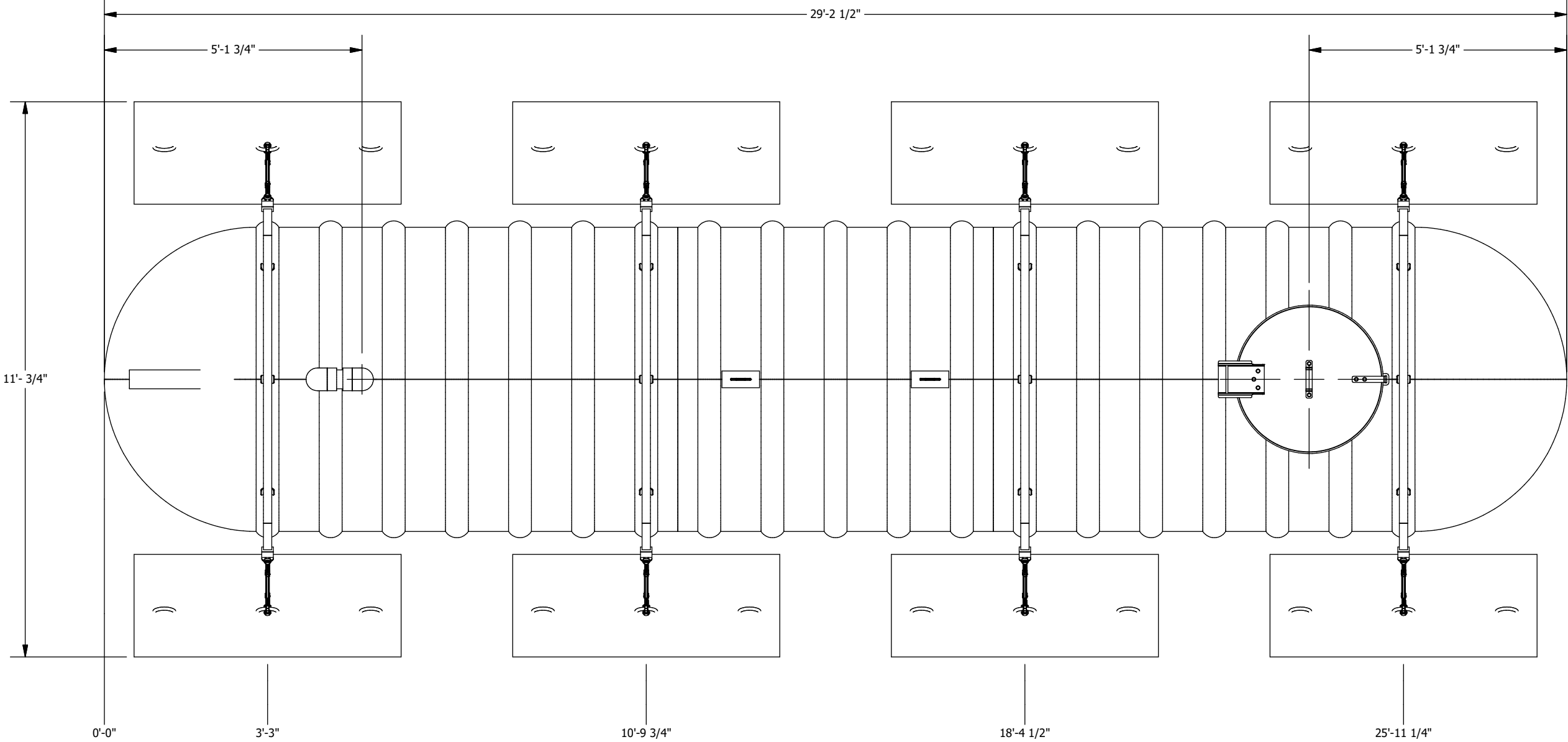
PLAN VIEW
