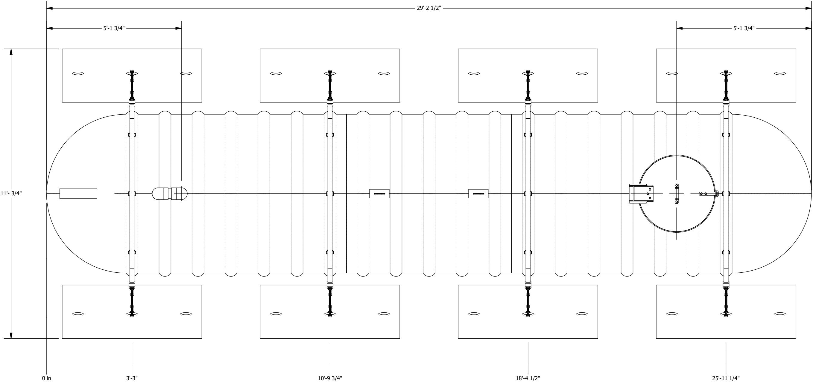
PLAN VIEW
