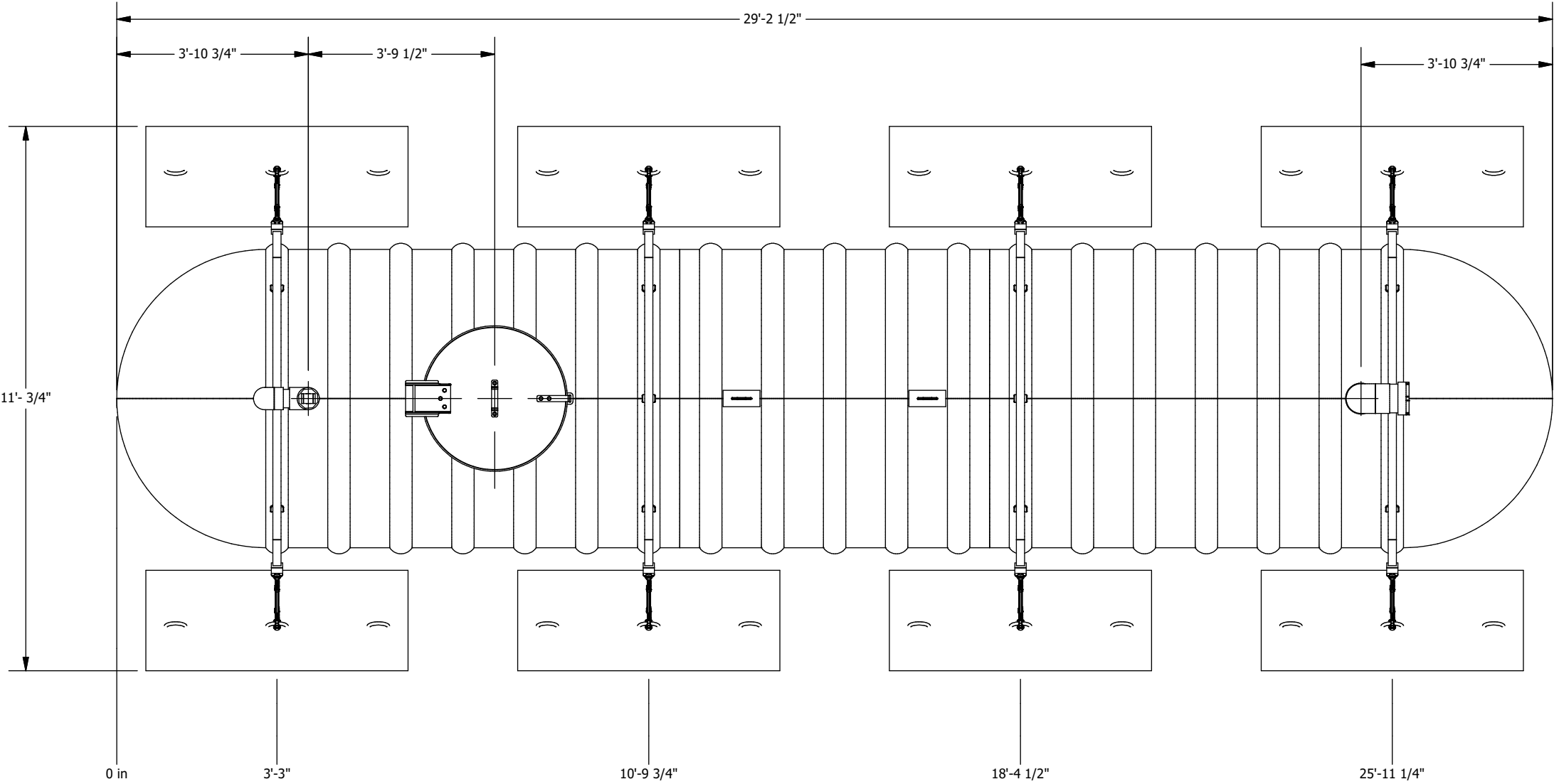
PLAN VIEW
