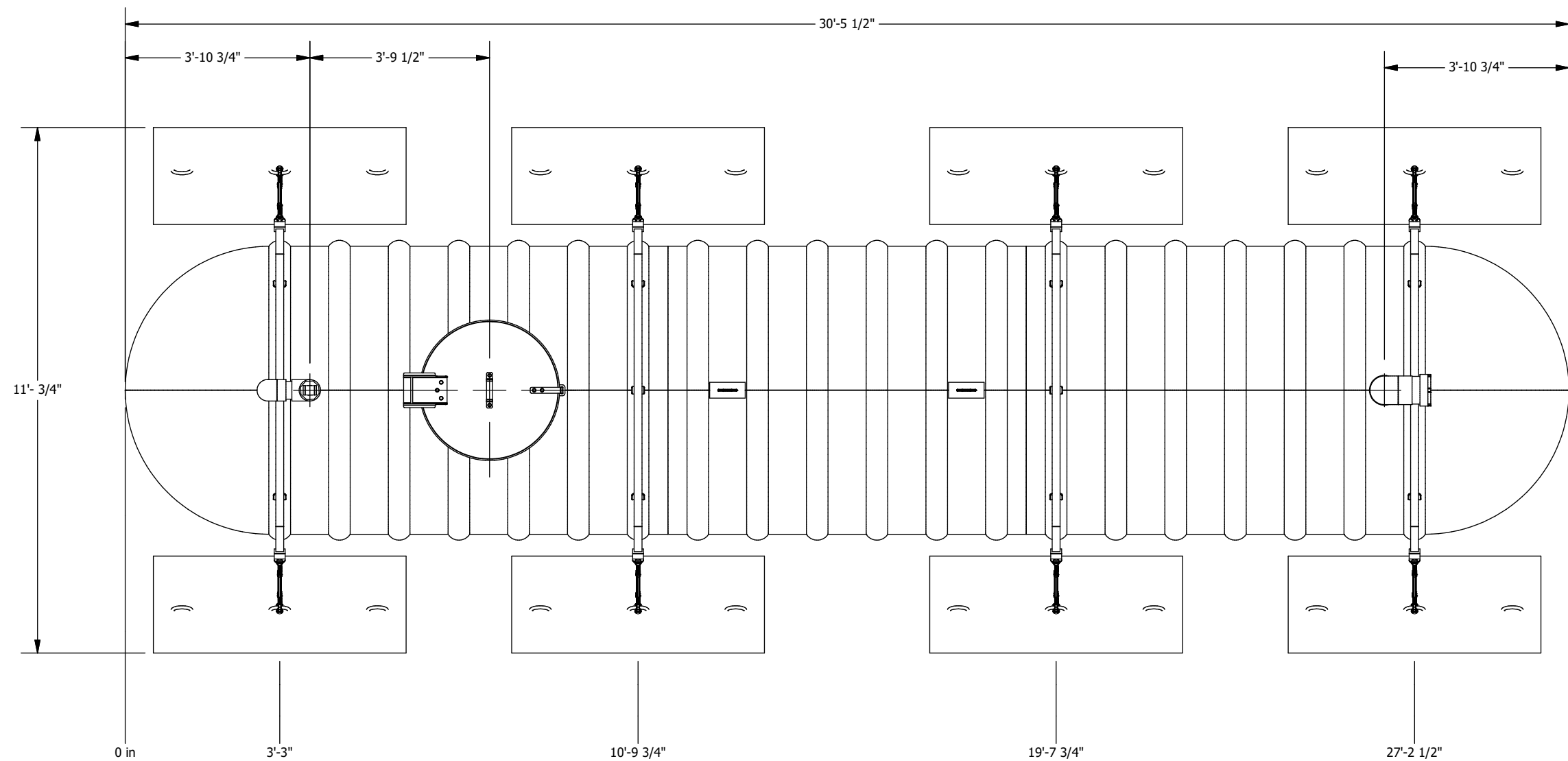
PLAN VIEW
