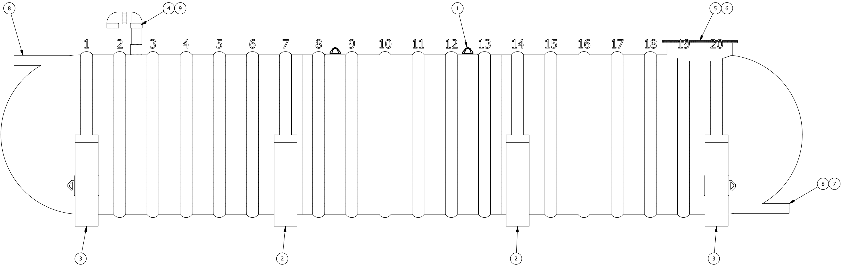
ELEVATION VIEW
