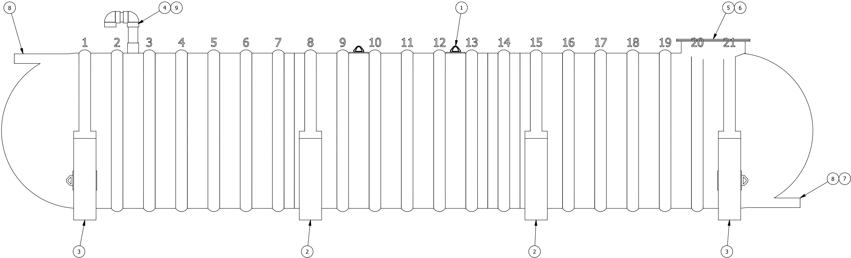
ELEVATION VIEW
