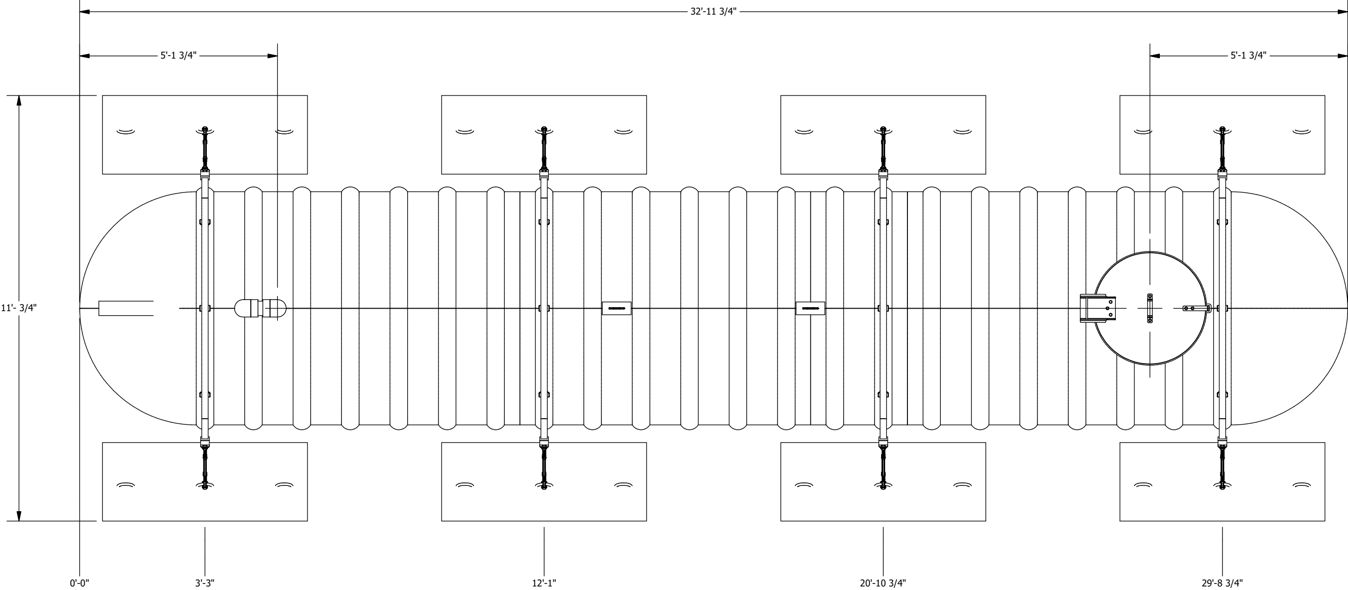
PLAN VIEW
