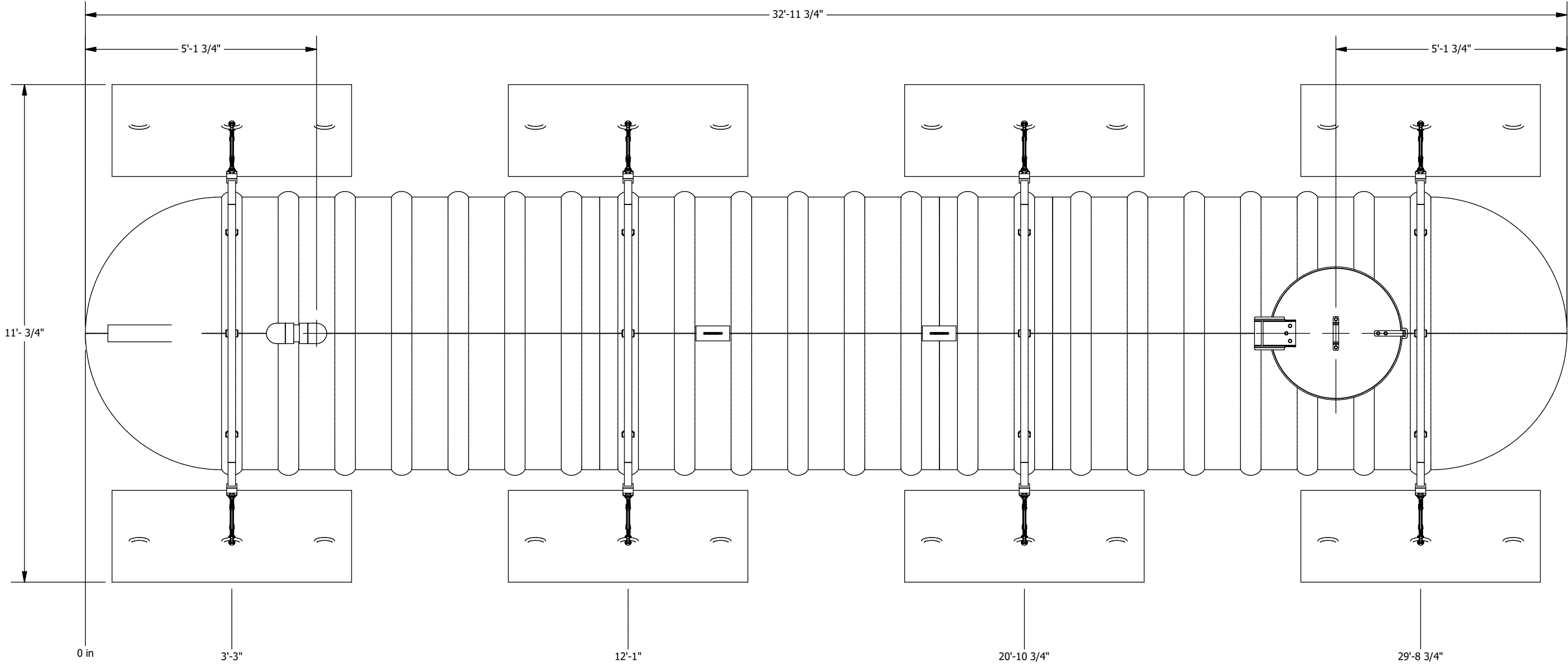
PLAN VIEW
