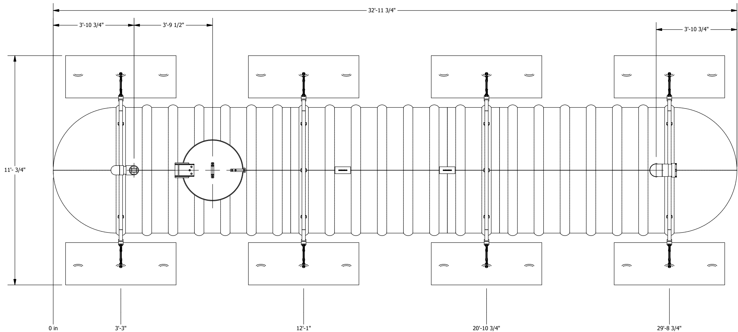
PLAN VIEW
