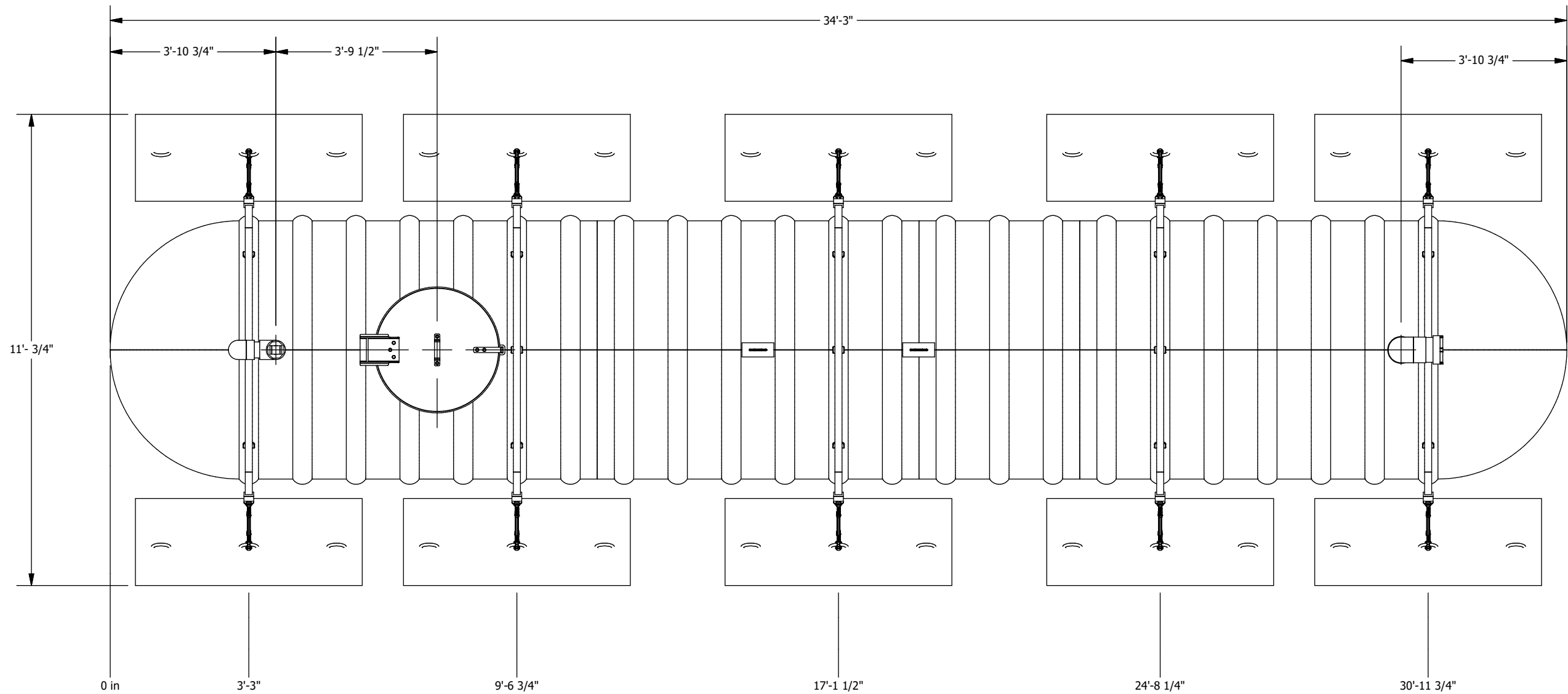
PLAN VIEW
