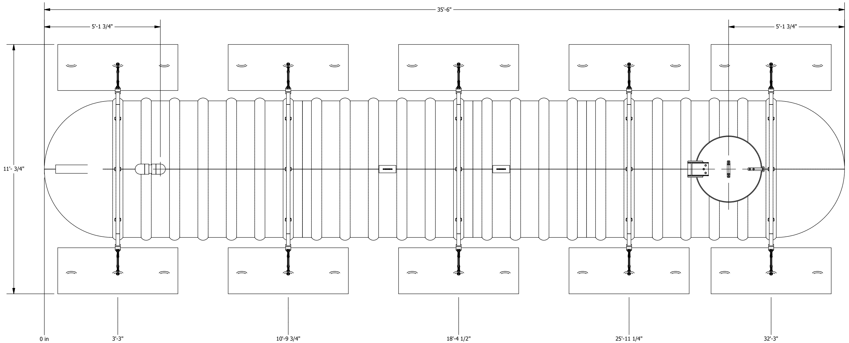
PLAN VIEW
