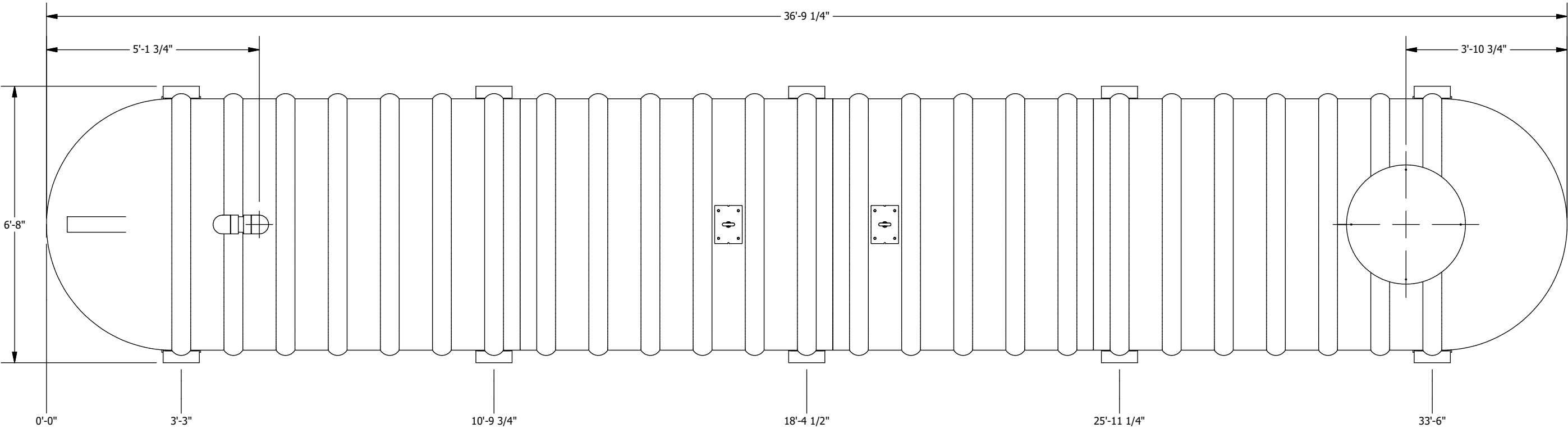
PLAN VIEW
