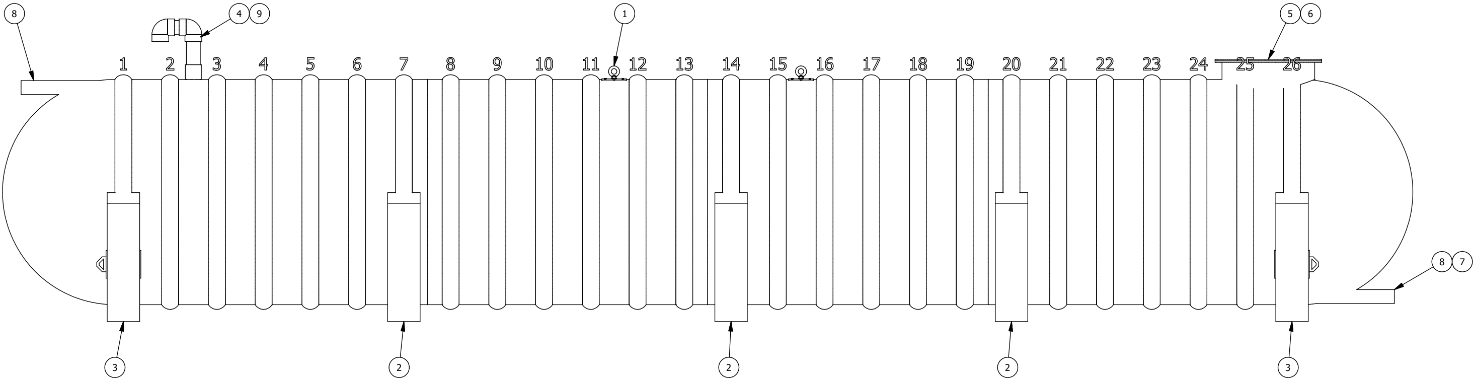
ELEVATION VIEW
