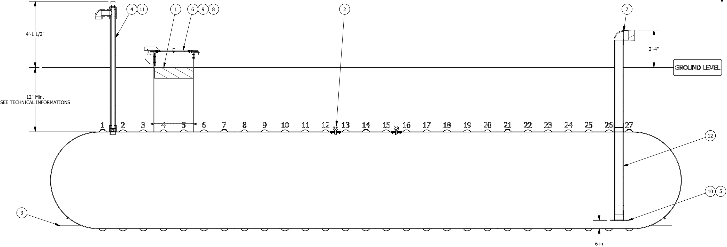
SECTION ELEVATION VIEW
