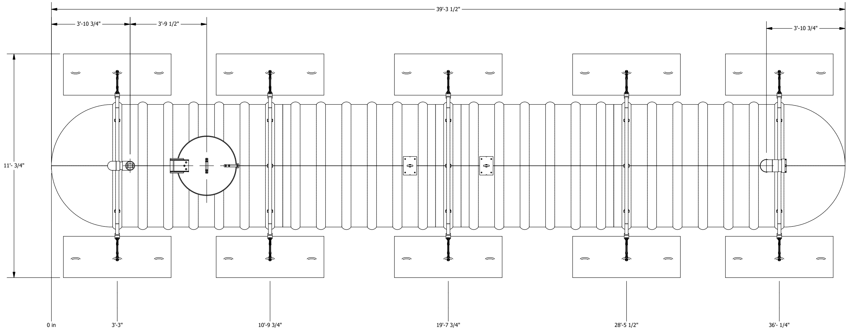
PLAN VIEW
