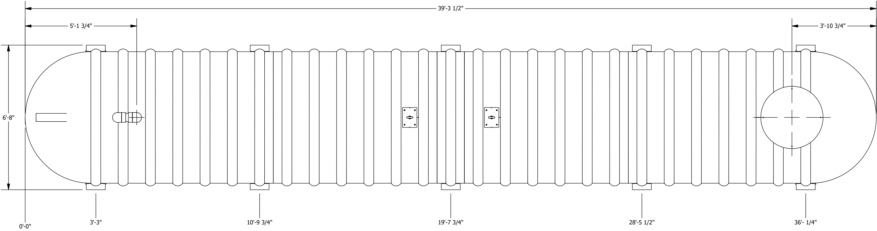
PLAN VIEW
