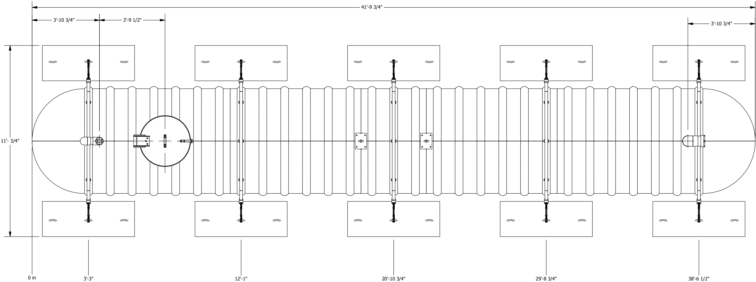
PLAN VIEW
