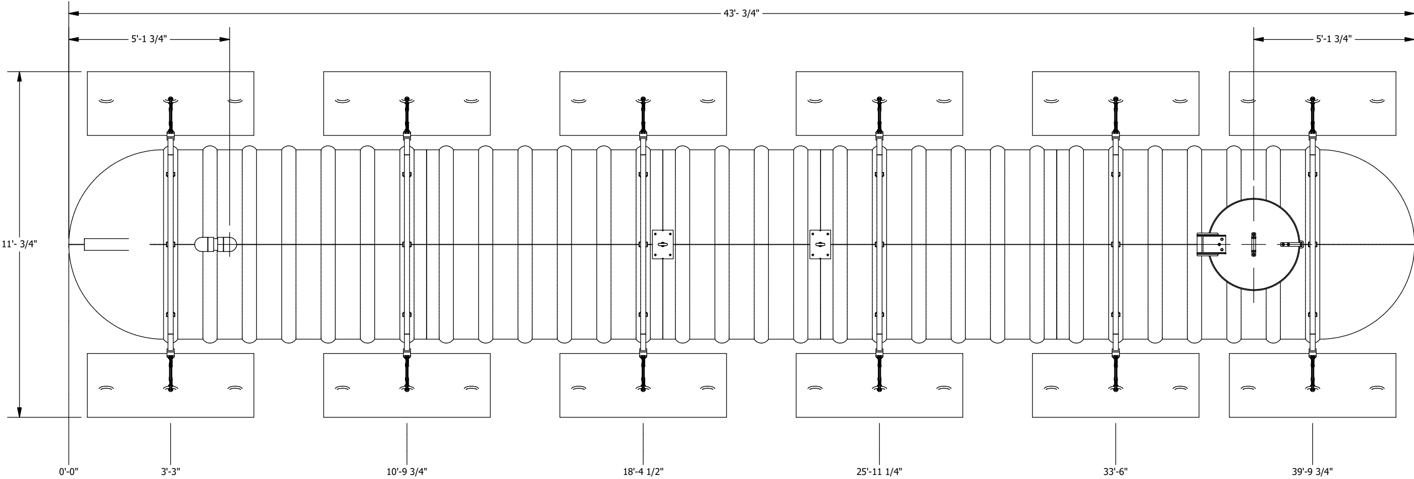
PLAN VIEW
