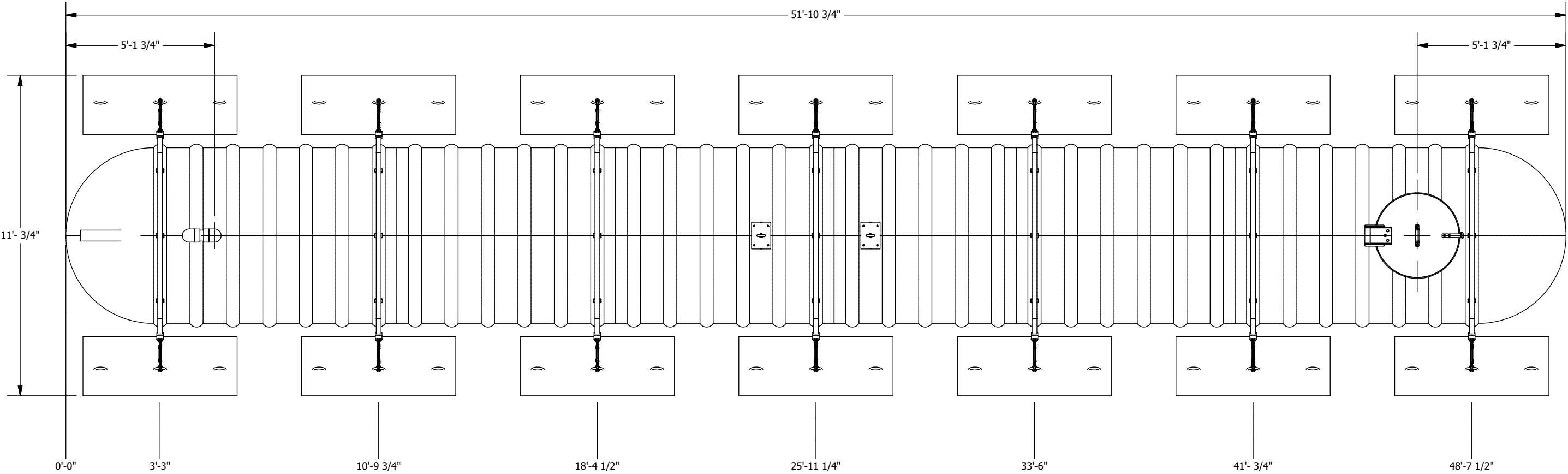
PLAN VIEW
