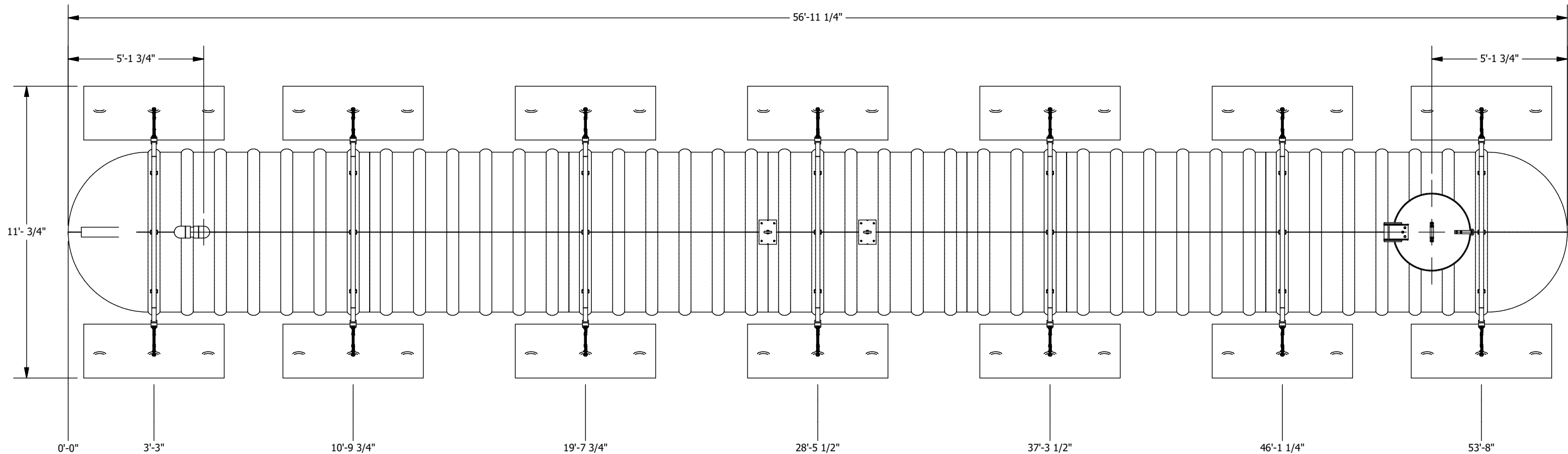
PLAN VIEW
