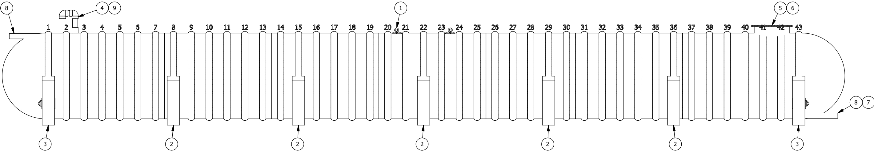
ELEVATION VIEW
