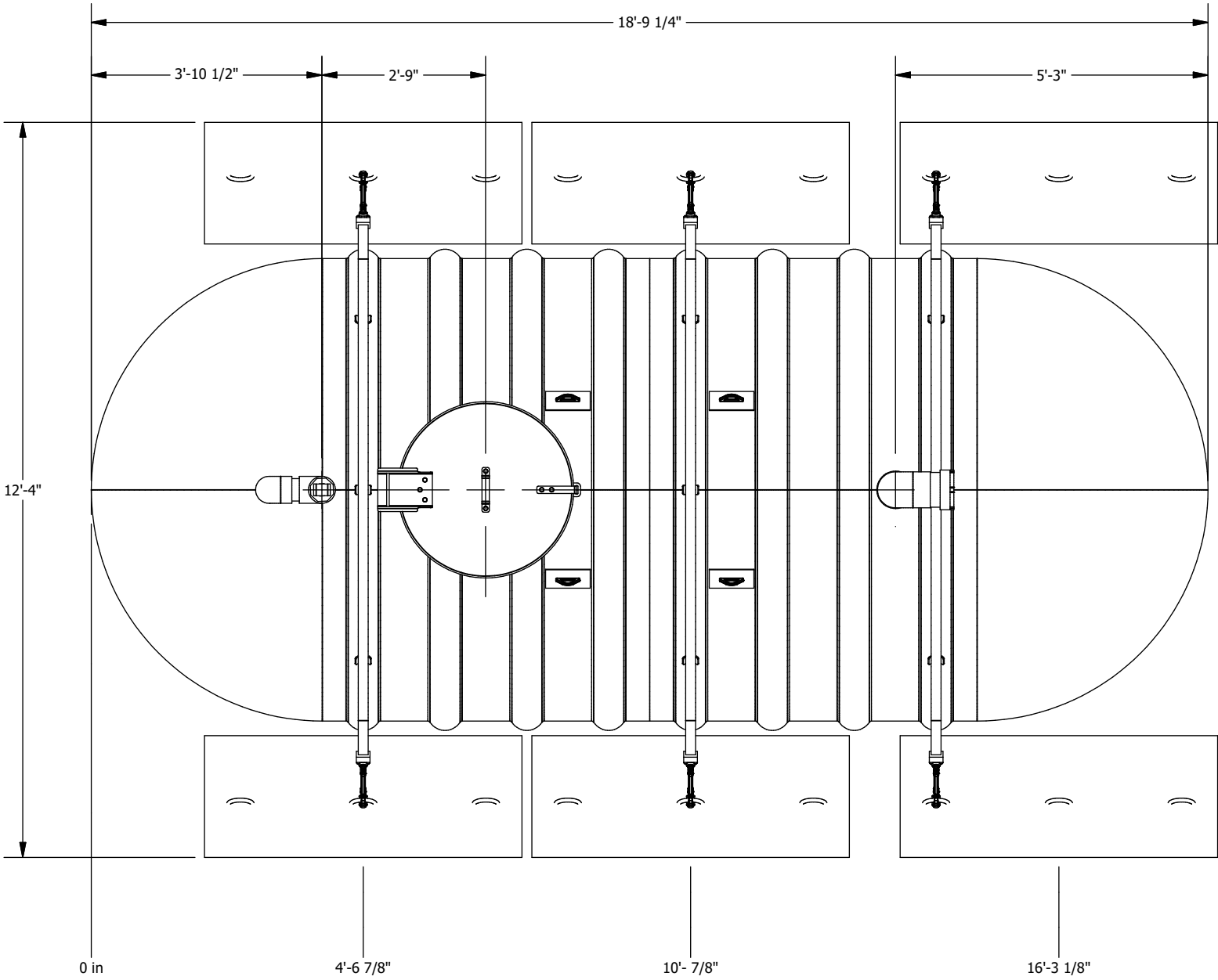
PLAN VIEW
