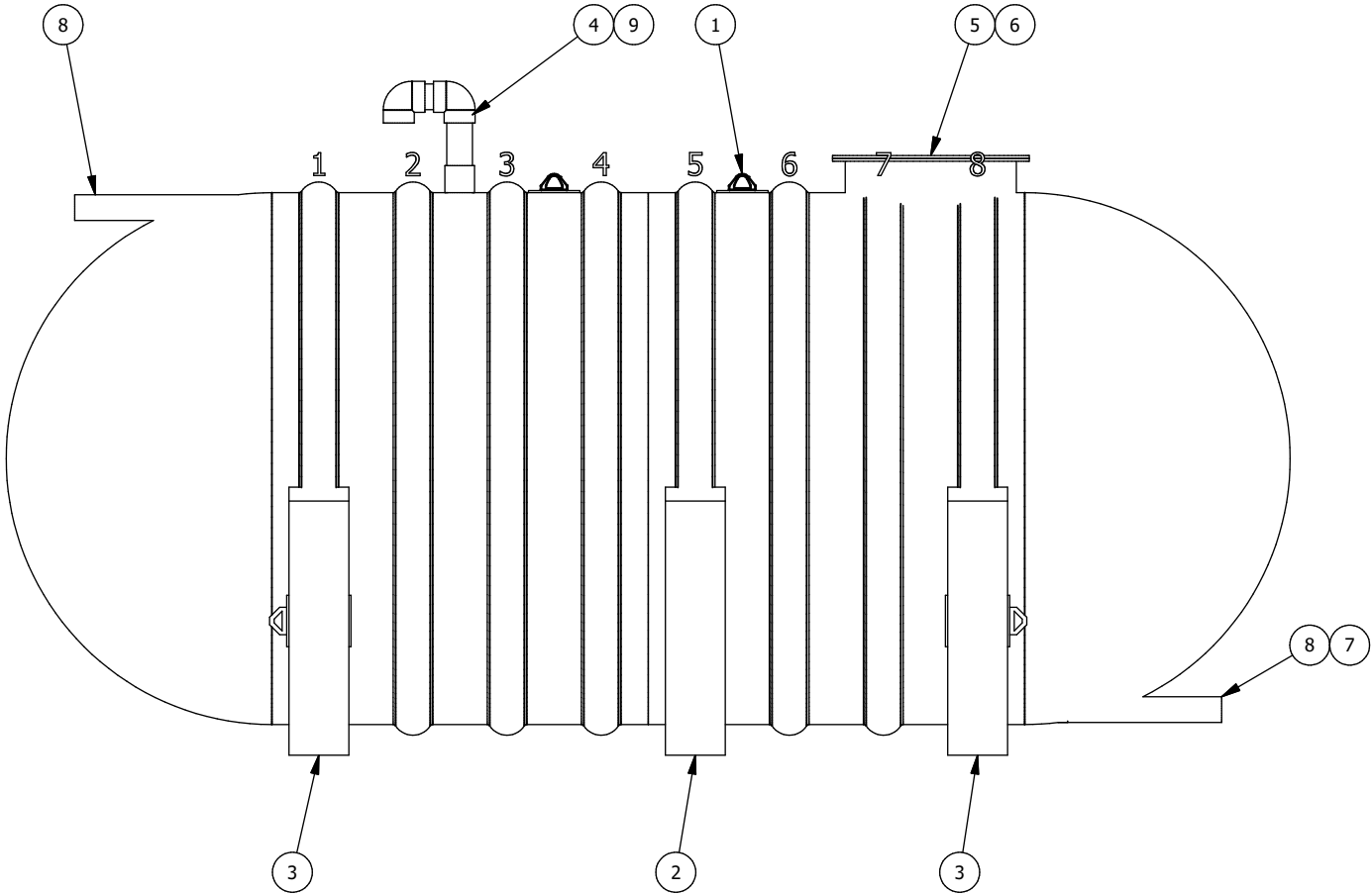
ELEVATION VIEW
