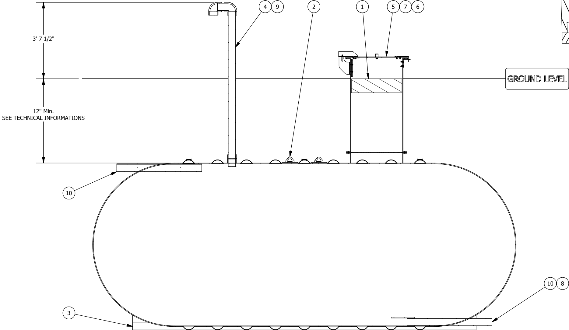
SECTION ELEVATION VIEW
