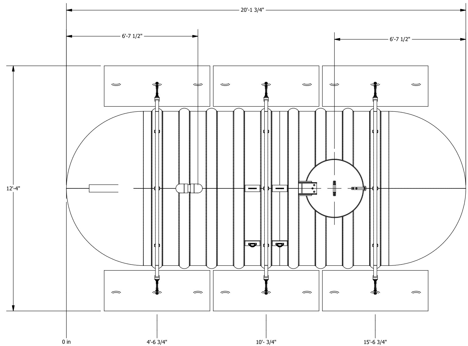
PLAN VIEW
