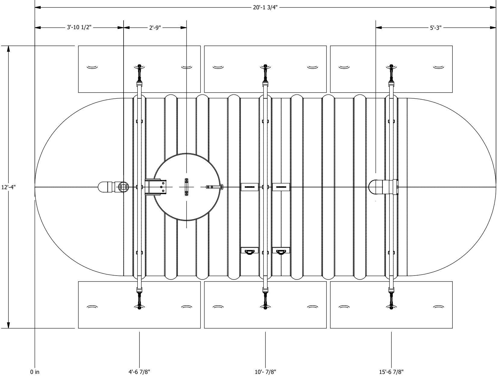
PLAN VIEW
