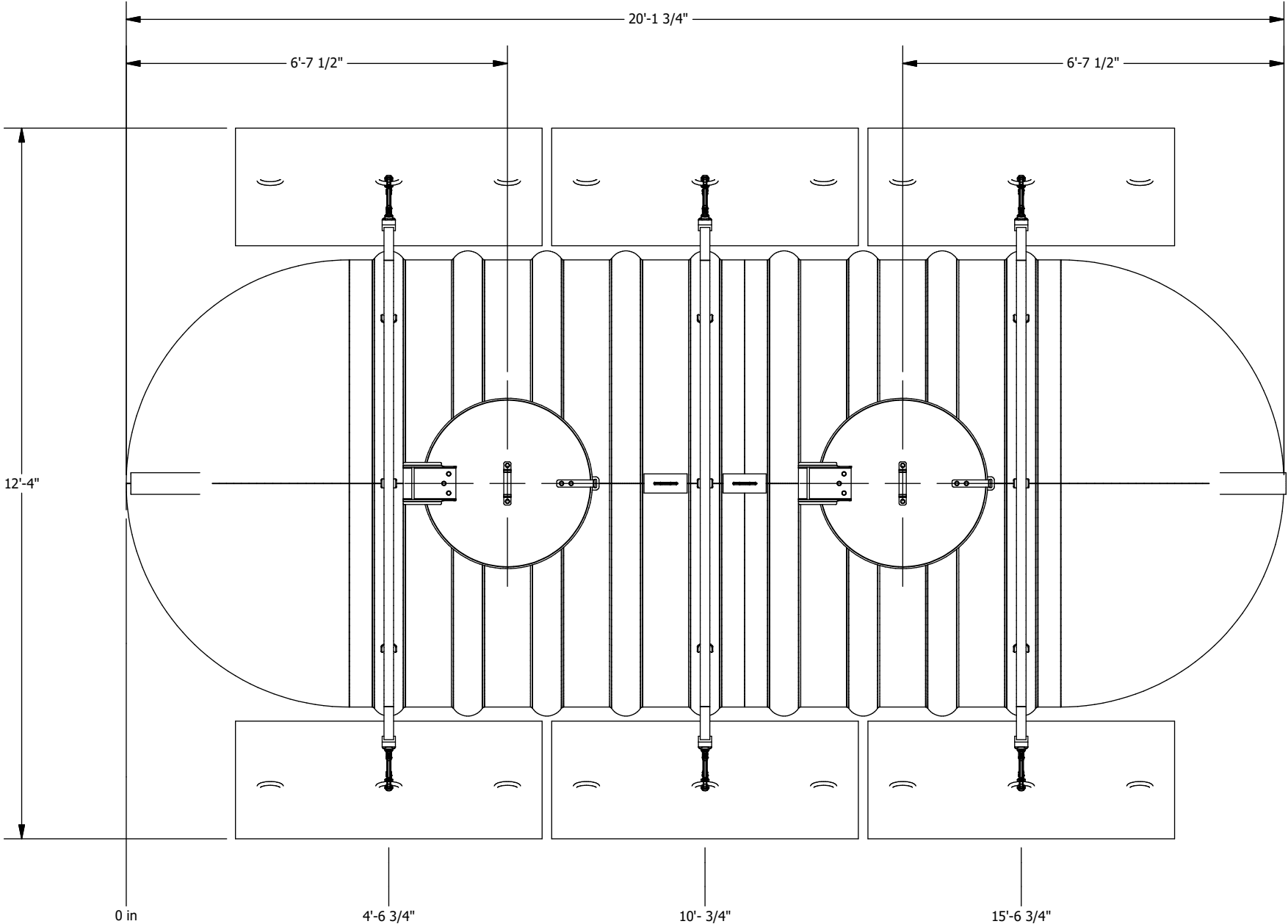
PLAN VIEW
