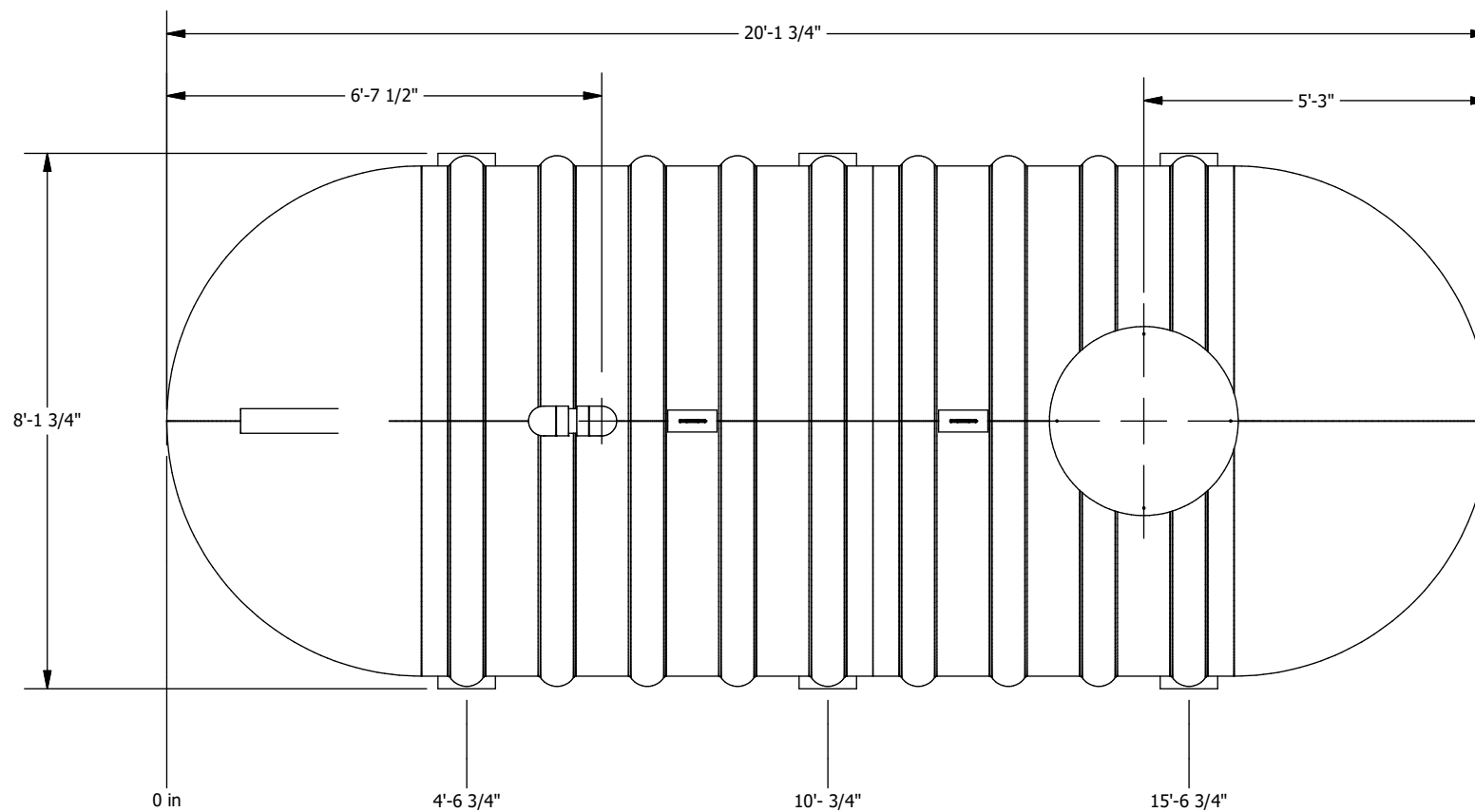
PLAN VIEW
