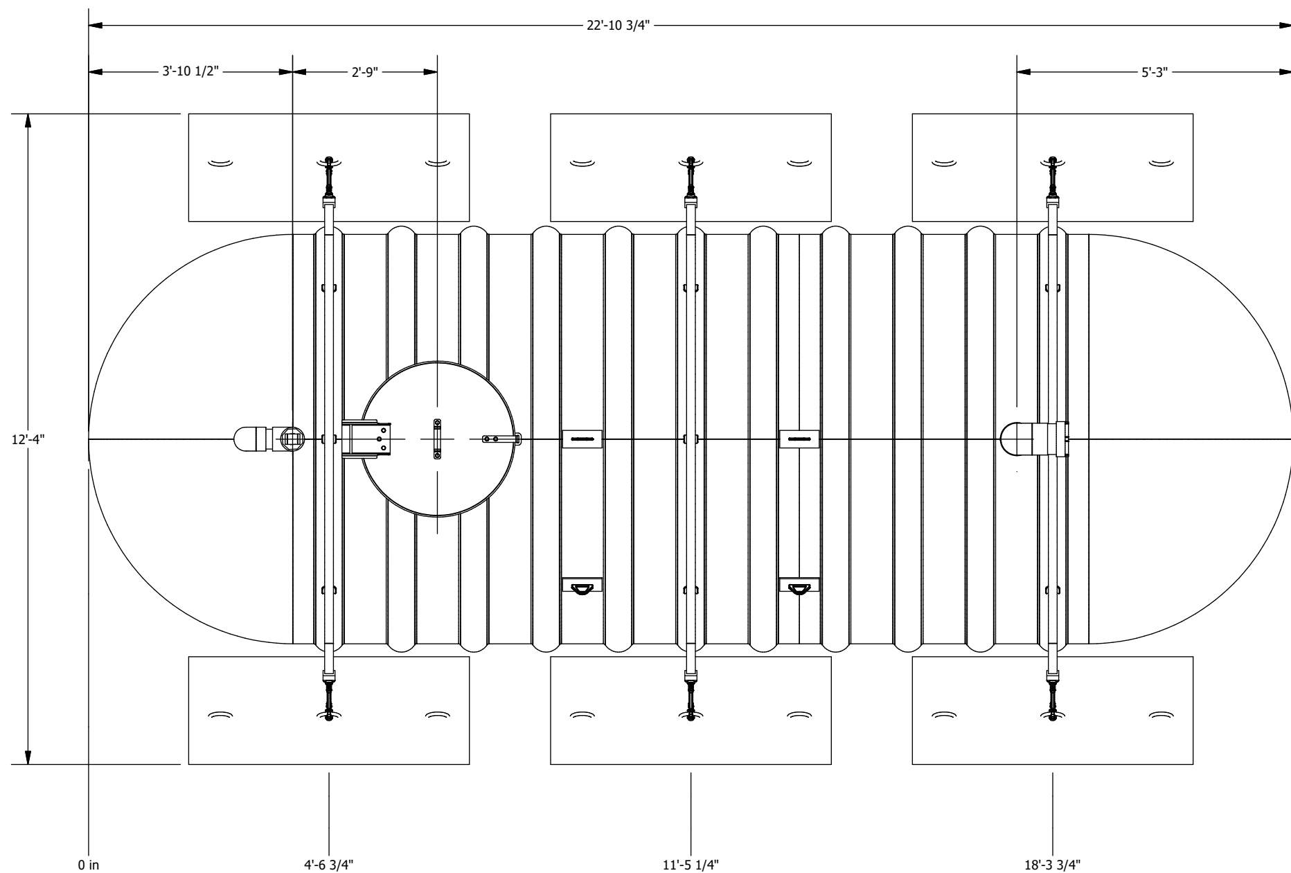
PLAN VIEW
