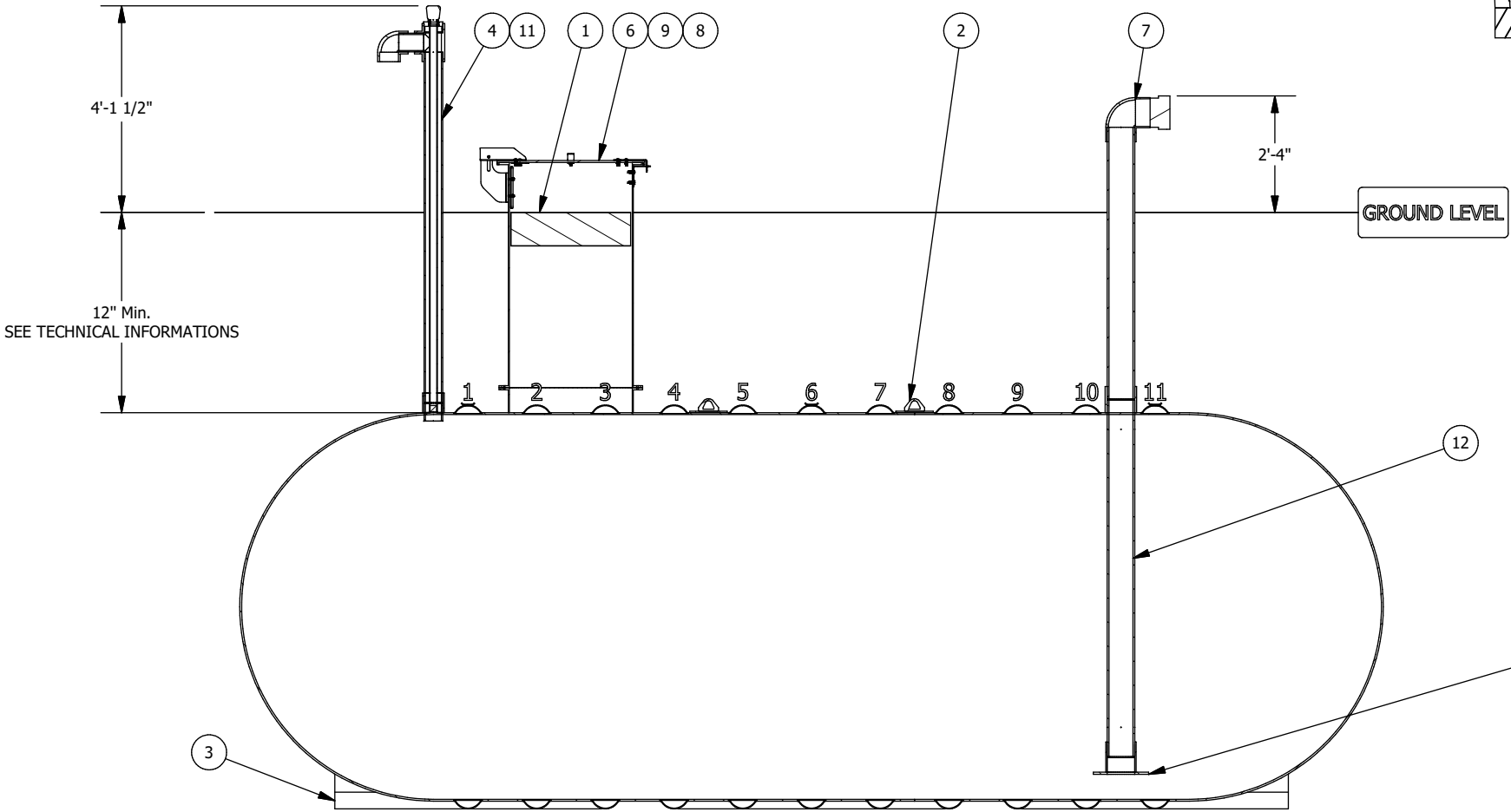
SECTION ELEVATION VIEW
