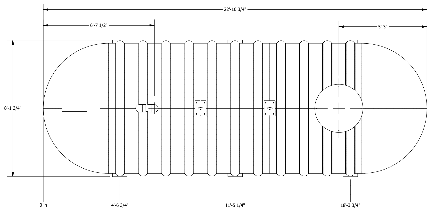
PLAN VIEW
